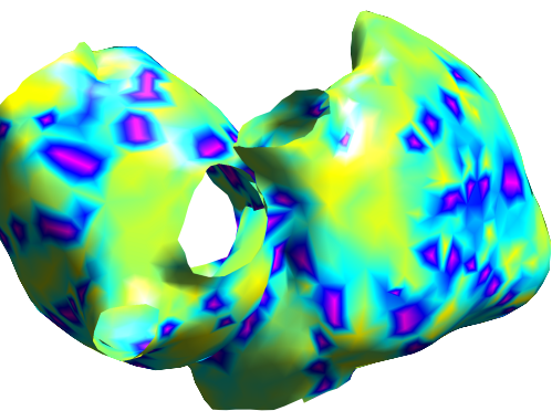
Interpolation
