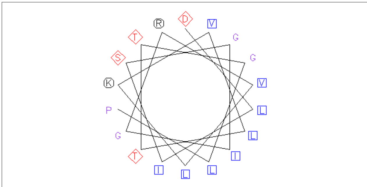
Figure 3.4: An example of an amino acid sequence plotted on a helical wheel. Aliphatic residues are shown as blue squares, polar or negatively charged residues as red diamonds, and positively charged residues as black octagons. The plot reveals whether hydrophobic amino acids are concentrated on one side of the helix, usually with polar or hydrophilic amino acids on the other. This arrangement is common in alpha helices within globular proteins, where one face of the helix is oriented toward the hydrophobic core and one face is oriented toward the solvent-exposed surface. ( Wikipedia )
