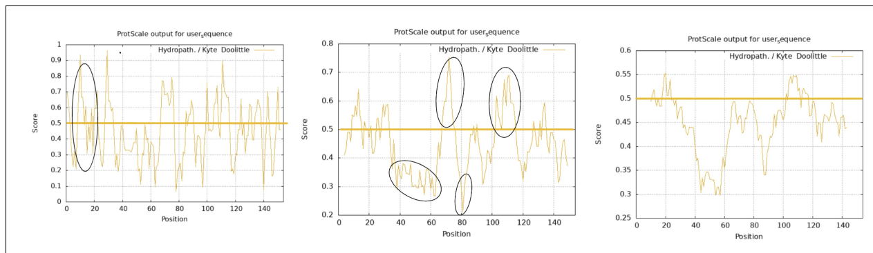
Figure 3.2: From left to right, window sizes of 3, 9, and 21. Center: medium window size. We can use this to get a grasp of how we expect the protein structure to be. For instance, we see two highly hydrophobic patches. We can reasonably expect that they correspond to the protein core. Also, we see some highly hydrophilic regions: these could be loops or coils that are highly exposed to the solvent and are connecting some secondary structures like \alpha -helices. Helices are expected to correspond to mildly hydrophobic patches. Left: decreasing the window size, we can spot precisely the signature of exposed \alpha -helices: they are marked by rapidly alternating hydrophilic and hydrophobic residues. This happens because a helix makes a complete turn every 3.6 aminoacids, and if it is found near the surface of the protein, it will have a side of more hydrophobic residues (the side that faces the protein core) and a side of more hydrophilic residues (the side that is exposed to the solvent).
