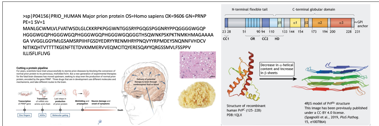
Figure 3.5: The Normal Form (PrP C ): Mostly alpha-helical and soluble. The Disease Form (PrP Sc ): It flips its structure to become mostly Beta-sheets. The "Infection": When a Beta-form prion touches a normal Alpha-form protein, it "convinces" (catalyzes) the Alpha-form to flip into a Beta-form. This is the "protein-based inheritance": it's an infection without DNA or a virus.
