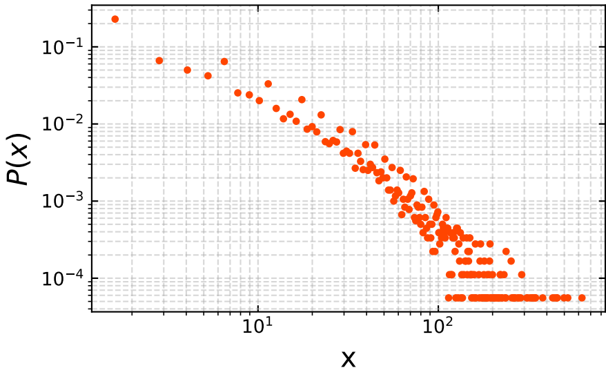
log-log plot with automated optimized x-axis binning, bin size = 1.22
