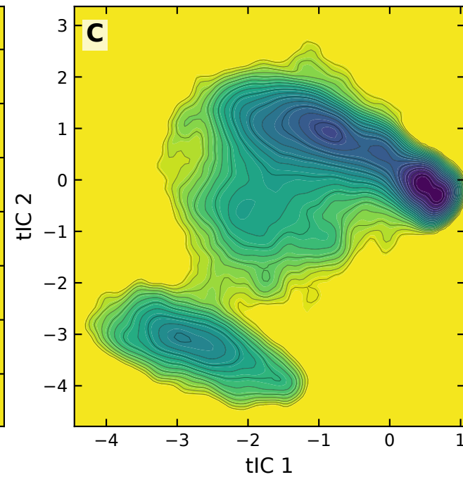
TICA dihedrals
