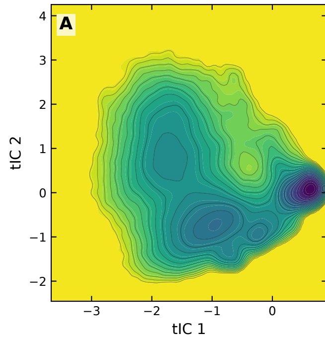
TICA distances
