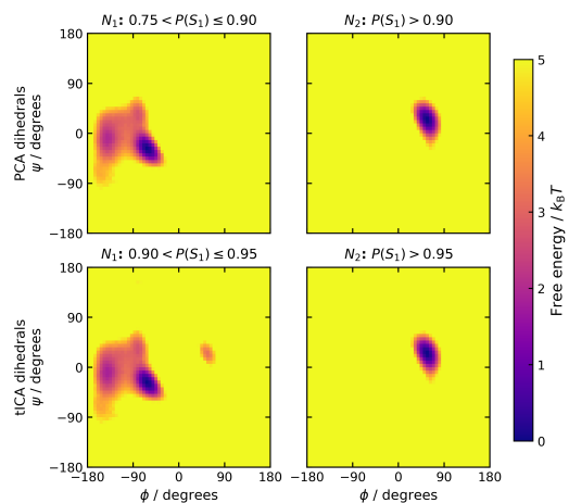
FIG. 6: Structural distinction between the two folded substates identified by the dihedral-based MSMs:
