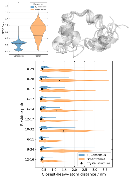
FIG. 5: Structural Analysis of S_1 consensus frames:
