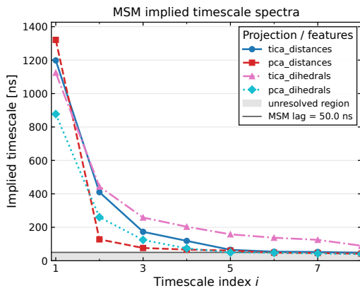
FIG. 4: Relaxation timescales spectra at selected lag time \tau = 50 ns. The horizontal grey line marks the MSM resolution limit ( t = \tau ).
