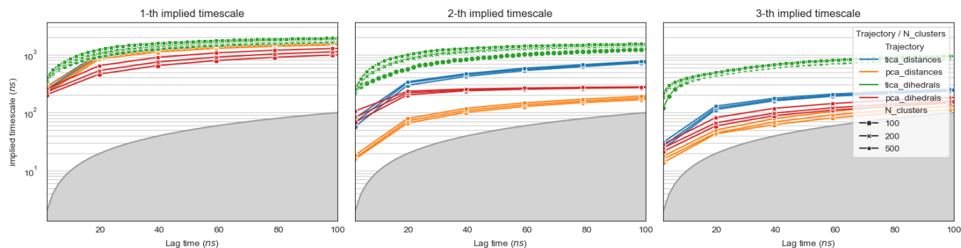
FIG. 2: Implied timescales convergence test. First three timescales. Colors distinguish the four combinations of features and dimensionality reduction method, marker styles distinguish the number of microstates used. Shaded grey area marks the region y \leq x . Any timescale falling in the shaded area is not resolved, referring to an equilibration process that happens in less than one evolution step of the Markov chain.
