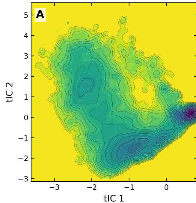
TICA distances
