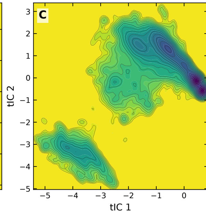
TICA dihedrals
