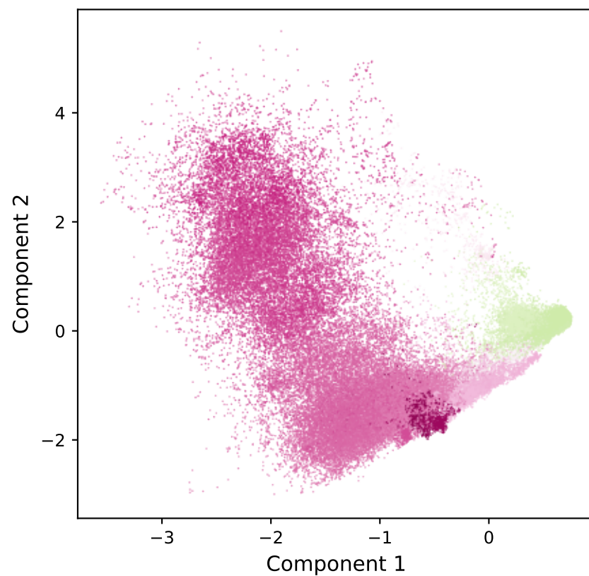
tica distances
