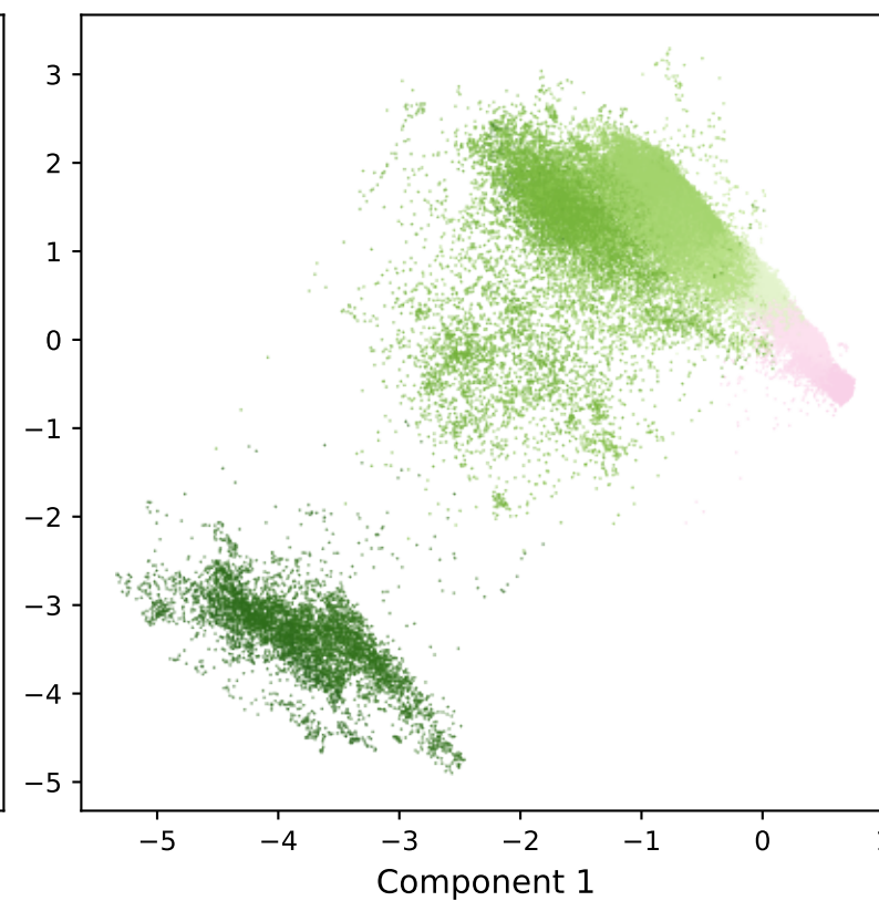
tica dihedrals
