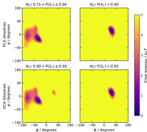
FIG. 5: Structural distinction between the two folded substates identified by the dihedral-based MSMs: (\phi, \psi) distribution of the residue Asp3 in the two subpopulations corresponding to the distinct minima observed within the folded basin.
