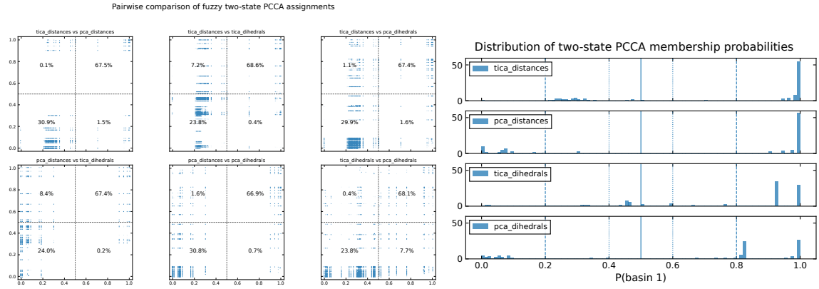
FIG. SF6: Fuzzy membership probabilities of the trajectory frames to the two macrostates across models. Left: Each panel shows the fuzzy membership probability of each frame in the trajectory to macrostate S_0 ( \simeq denatured basin) and macrostate S_1 ( \simeq folded basin) for a different model. The models based on distances (tica-distances and pca-distances) show very similar distributions, while the tica-dihedrals model exhibits a broader distribution, particularly for frames assigned to the denatured basin. This indicates that the tica-dihedrals model has more uncertainty in assigning frames to the denatured basin. Right: Distribution of the fuzzy membership probability of each frame to macrostate 1 for the four MSMs. Probabilities close to 0 or 1 correspond to frames that are confidently assigned to a single macrostate.
