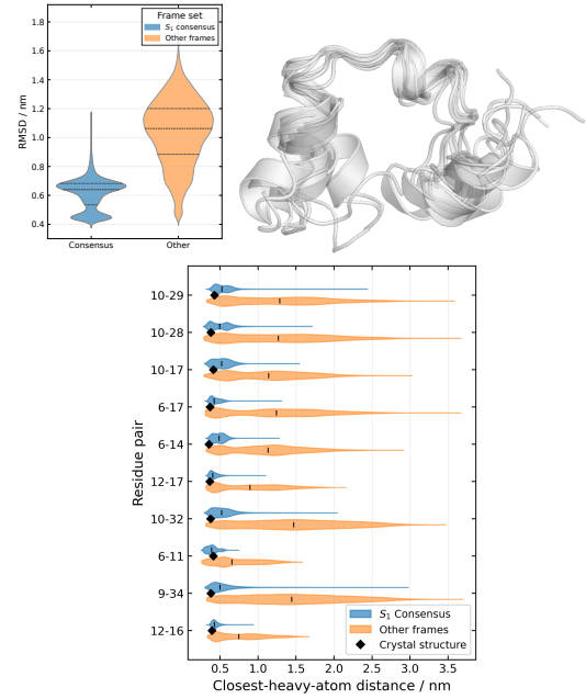
FIG. 4: Structural Analysis of S_1 consensus frames: Top left: distribution of RMSD from the crystal structure. Top right: overlay of a random ensemble of 8 consensus frames. Bottom: distribution of most important contacts as identified by the score defined in the text.
