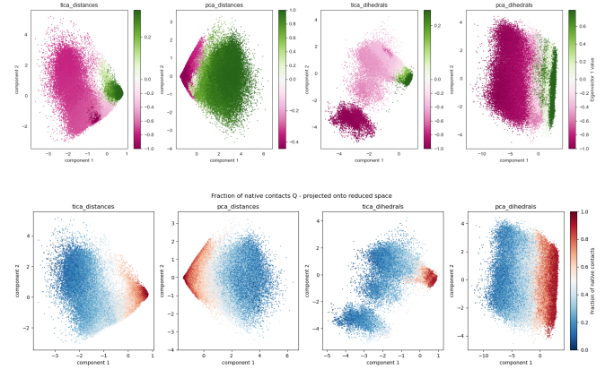
FIG. 5: Comparison between the slowest MSM relaxation mode and a structural folding descriptor. Top row: values of the first non-trivial eigenvector projected onto the first two components of the reduced coordinate space. Positive and negative components identify regions that exchange probability on the slowest resolved timescale of the Markov model. Bottom row: projection of the fraction of native contacts, Q , onto the same coordinates. The close correspondence between the eigenvector sign pattern and the distribution of Q indicates that the slowest kinetic process captured by the MSM is associated with the folding-unfolding transition.
