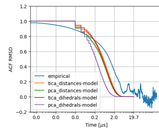
FIG. 3: Results of the autocorrelation test: Autocorrelation function of the root mean square deviation (RMSD) from the crystal structure, as obtained from the molecular dynamics trajectory (blue) and predicted by the four MSMs (orange, green, red and purple). TODO: add uncertainties using bootstrapping
