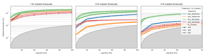
FIG. 2: Implied timescales convergence test. First three implied timescales as a function of the MSM lagtime. Colors denote the four combinations of feature set and dimensionality reduction method, while marker styles indicate the number of microstates used in the state-space discretization. The shaded region corresponds to t_i \leq \tau , where t_i is the implied timescale and \tau the MSM lagtime. Timescales falling within this region are not resolved by the model, as the associated relaxation process occurs on a timescale shorter than a single Markov-chain transition step. TODO: make fig more readable, maybe split into rows TODO: add uncertainties using bootstrapping
