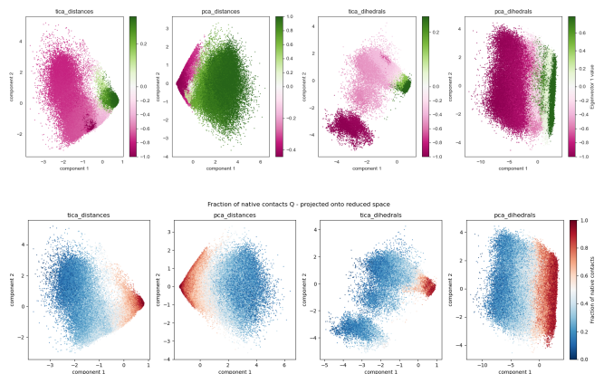
FIG. 4: Comparison between the slowest MSM relaxation mode and a structural folding descriptor. Top row: values of the first non-trivial eigenvector projected onto the first two components of the reduced coordinate space. Positive and negative components identify regions that exchange probability on the slowest resolved timescale of the Markov model. Bottom row: projection of the fraction of native contacts, Q , onto the same coordinates. The close correspondence between the eigenvector sign pattern and the distribution of Q indicates that the slowest kinetic process captured by the MSM is associated with the folding-unfolding transition.
