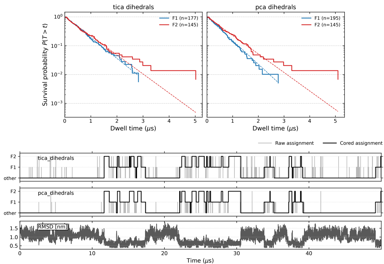
FIG. SF10: Manual analysis of dihedral-resolved substates.
