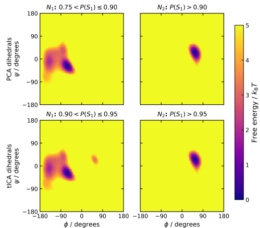
FIG. 6: Structural distinction between the two folded substates identified by the dihedral-based MSMs: (\phi, \psi) distribution of the residue Asp3 in the two subpopulations corresponding to the distinct minima observed within the folded basin.
