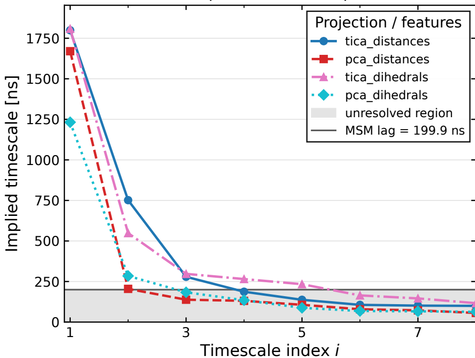
MSM implied timescale spectra
