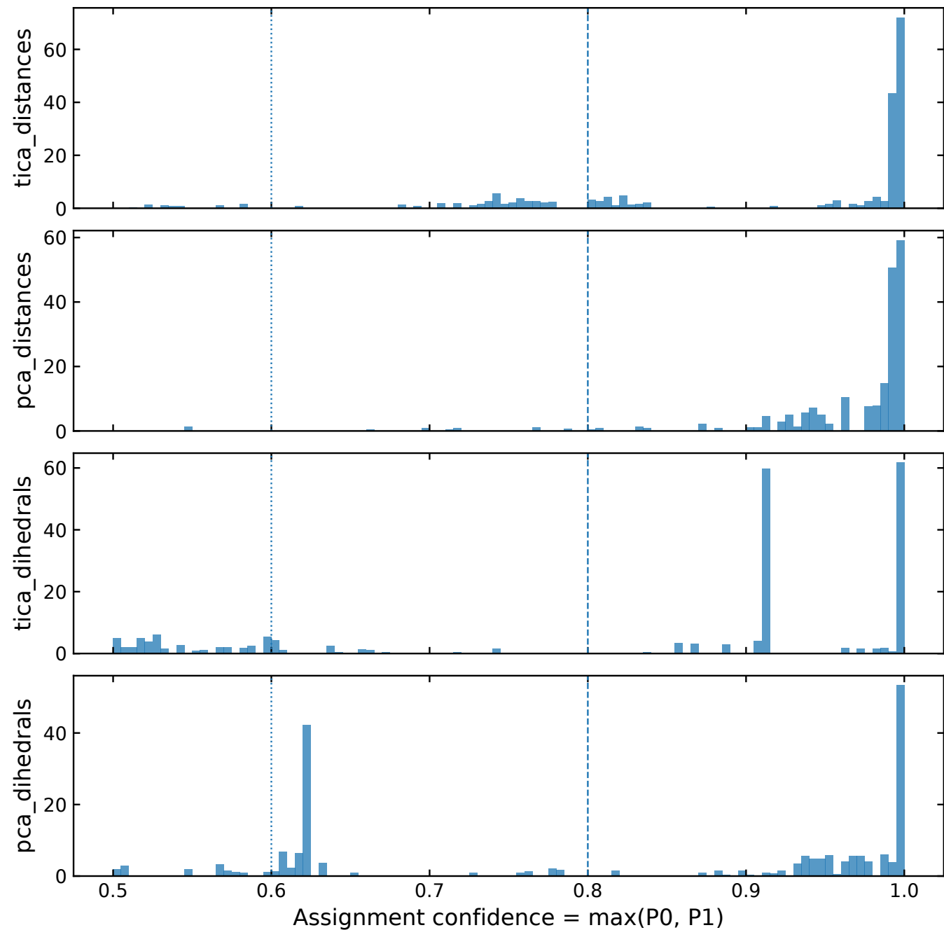
Sharpness of two-state PCCA assignments
