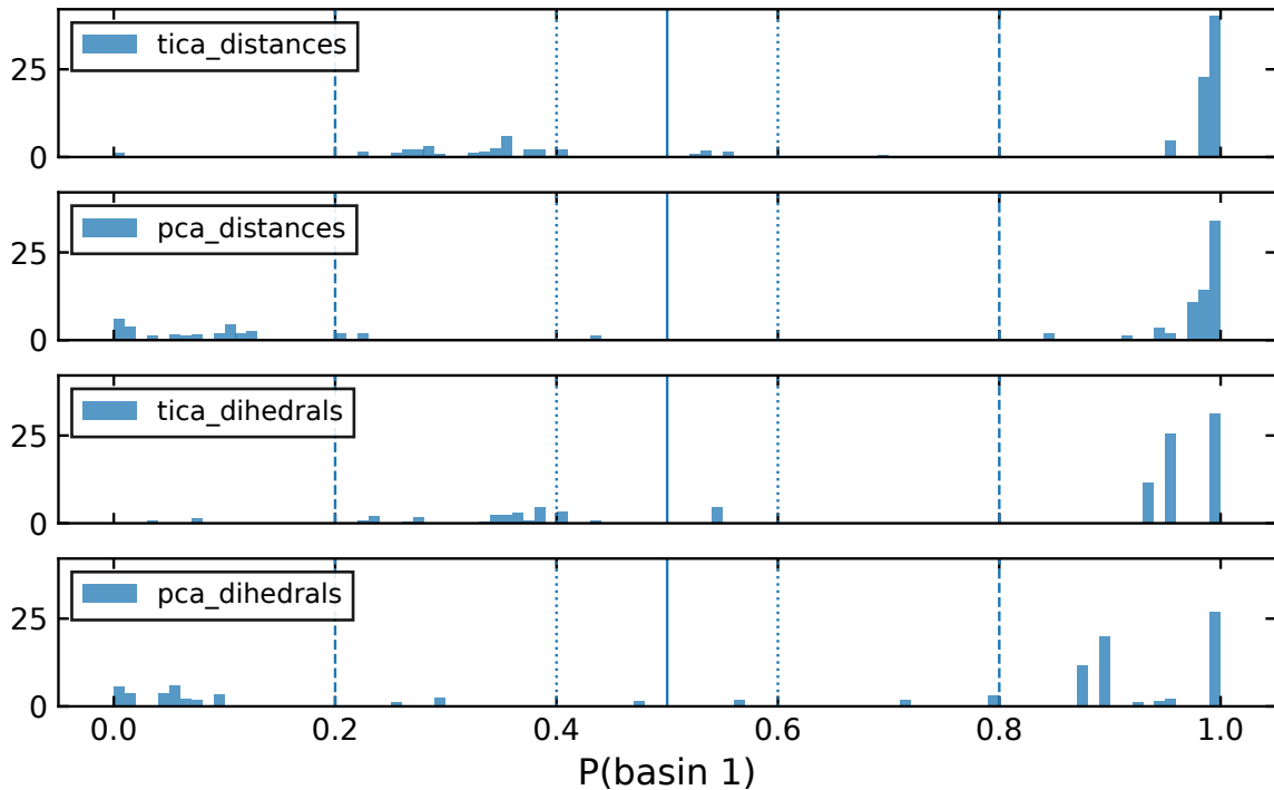
Distribution of two-state PCCA membership probabilities
