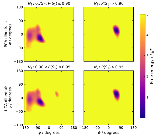
FIG. 6: Distribution of dihedral angles of Asp3 in the two sets of microstates individuated by dihedral-based MSMs.
