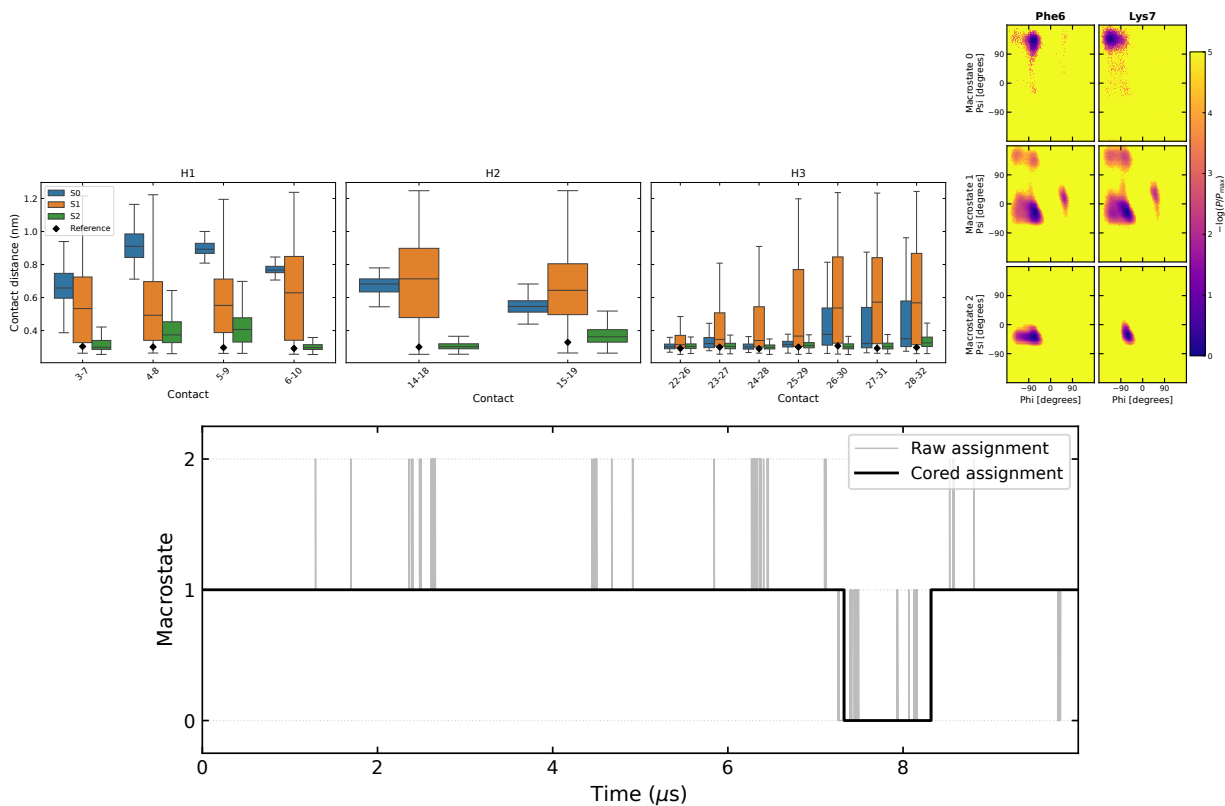
FIG. SF9: Trajectory of the three-state PCCA++ model for tICA-distances.
