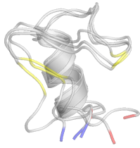
FIG. 8: Representative structure of macrostate S_0 of the tICA-distances three-state PCCA++ model. Helix 3 is formed, while helix 1 is completely extended.
