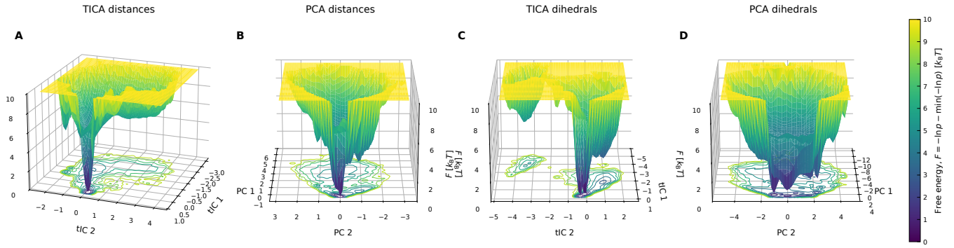
FIG. 2: Although free energy projections must be taken with care and can be potentially misleading, it is evident that the four pipelines reconstruct landscapes that look very different. In particular, dihedrals identify two global minima, while distances identify only one. tICA also produces much higher gaps in the free energy between what should represent the folded and unfolded basin and both tica show a basin that has low free energy and is isolated from the main funnel.
