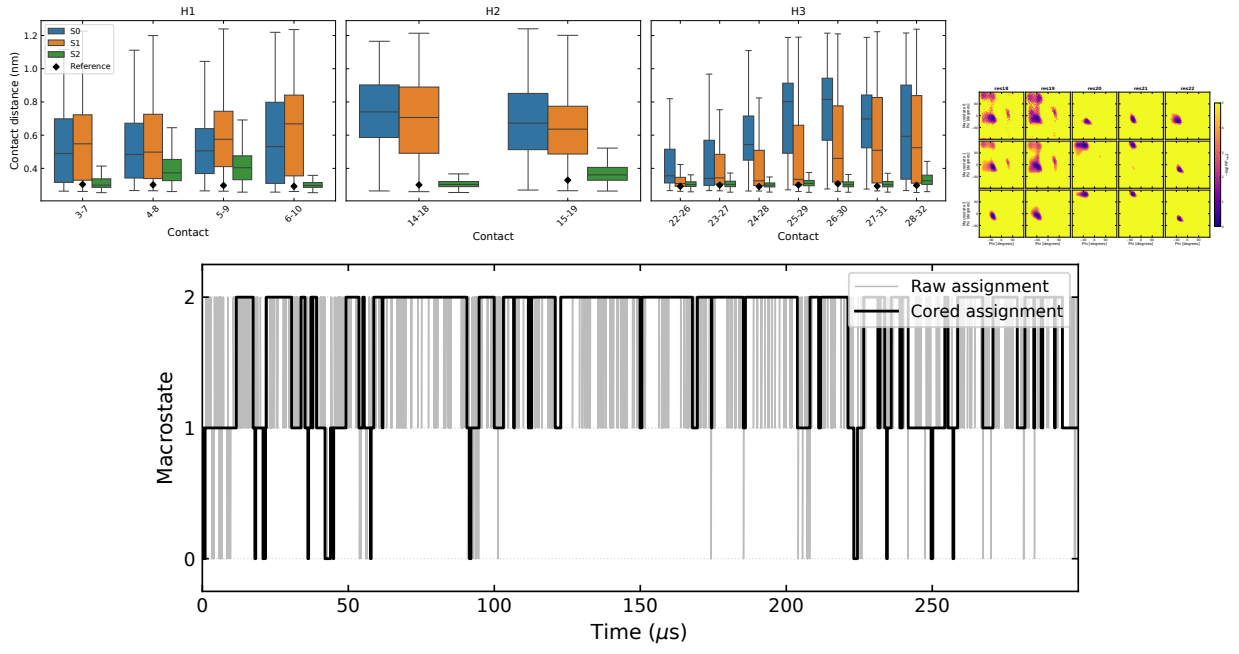
FIG. SF10: Trajectory of the three-state PCCA++ model for tICA-dihedrals.
