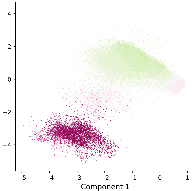
MSM dynamical mode 2 projected onto TICA coordinates
