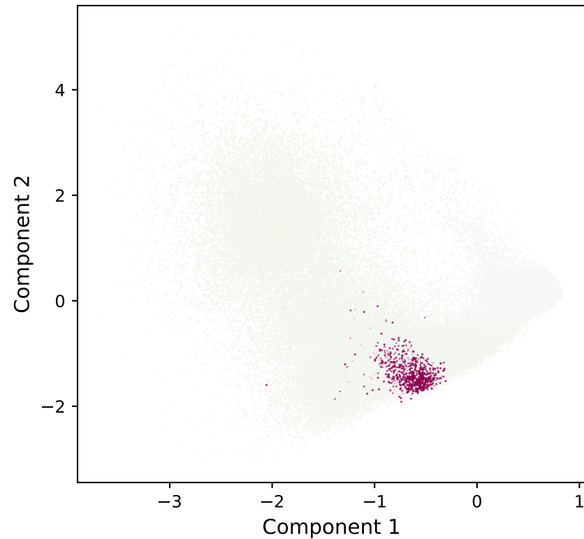
MSM dynamical mode 2 projected onto TICA coordinates
