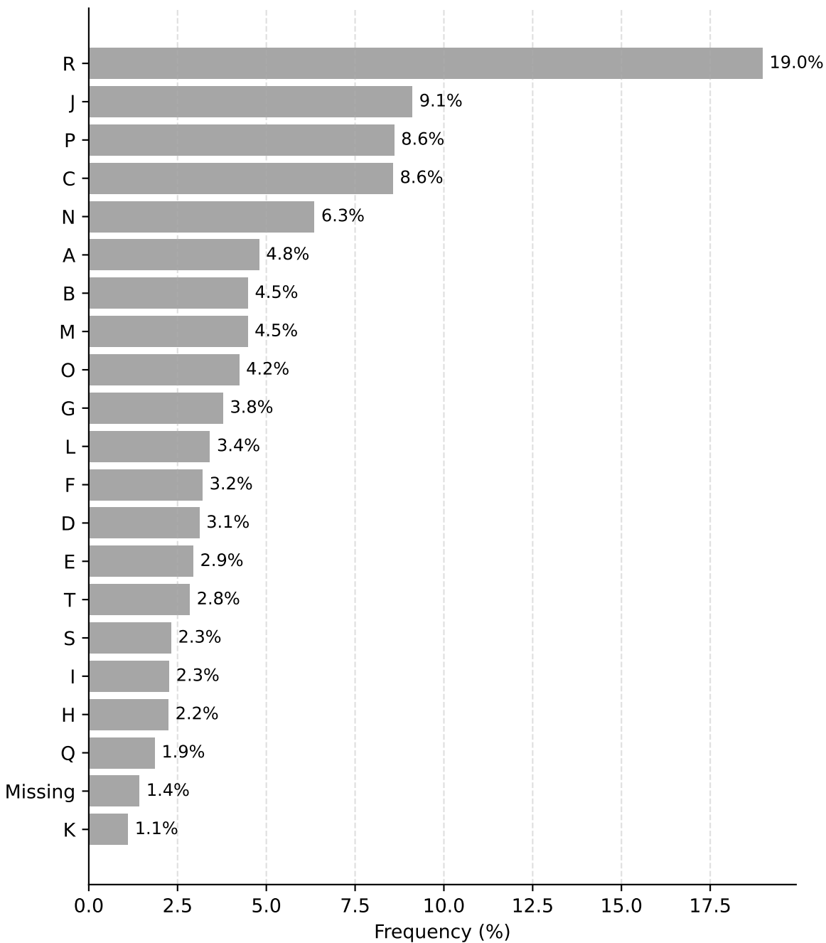
Distribution of Foldseek 3Di state
