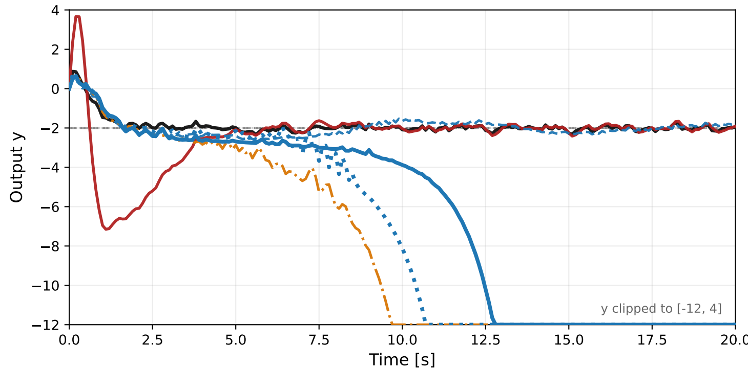
Noise scale x = 3 newly failing: \text{MLP}_r(16,16) , \text{MLP}_r(32,32,32)
