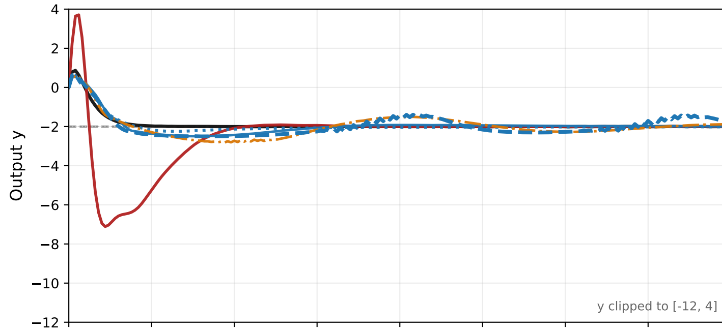
Noise scale x = 0.1 newly failing: \text{MLP}_r(32,32)
