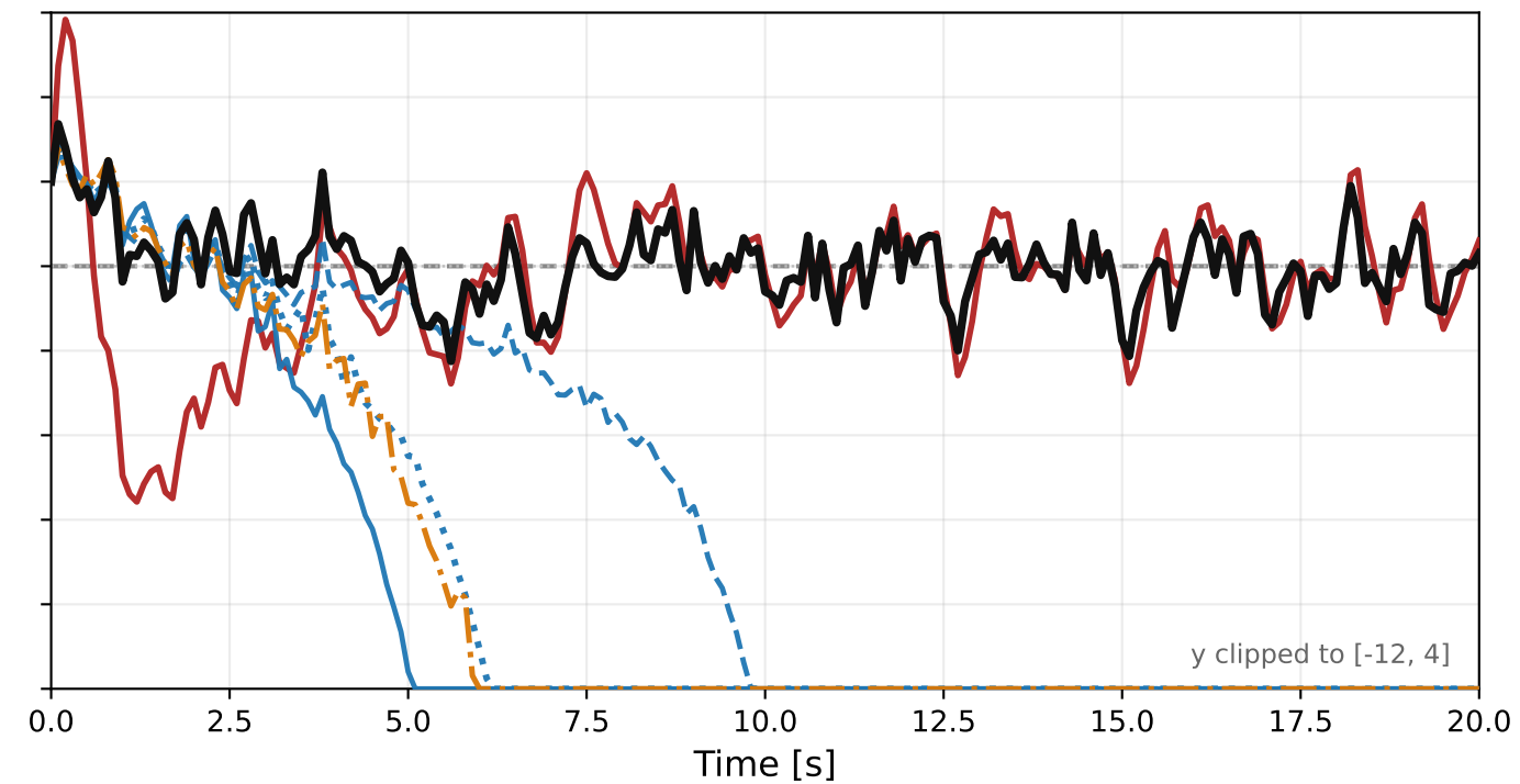
Noise scale x = 20 highest tested scale; MPC still passes all plants
