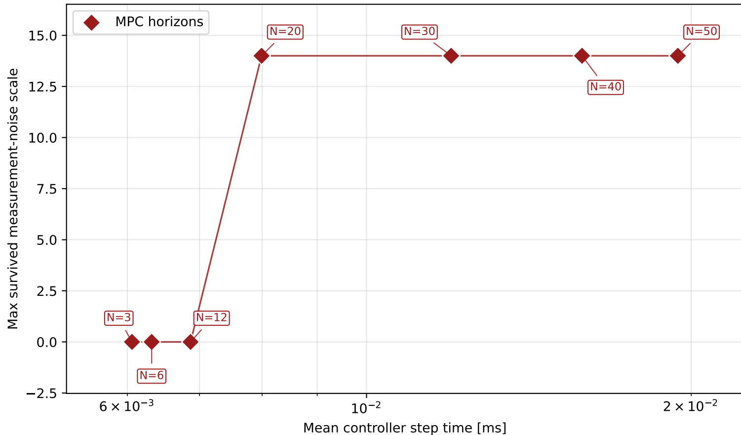
MPC runtime vs measurement-noise robustness
