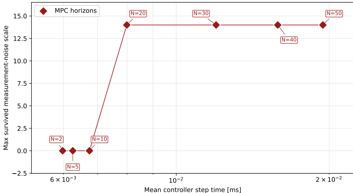
MPC runtime vs measurement-noise robustness
