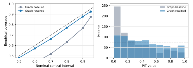
FIGURE 7. T_0 \rightarrow T_3 reliability and PIT diagnostics for the baseline and final retained graph MC distributions. The final retained model improves central-interval coverage across nominal levels and makes the PIT distribution less boundary-concentrated.
