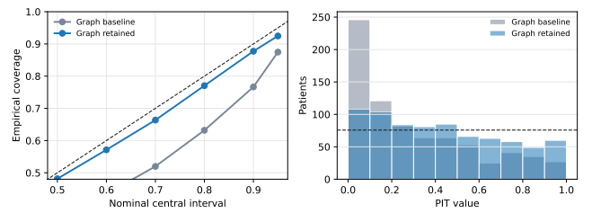
FIGURE 7. T_0 \rightarrow T_3 reliability and PIT diagnostics for the baseline and final retained graph MC distributions. The final retained model improves central-interval coverage across nominal levels and makes the PIT distribution less boundary-concentrated.
