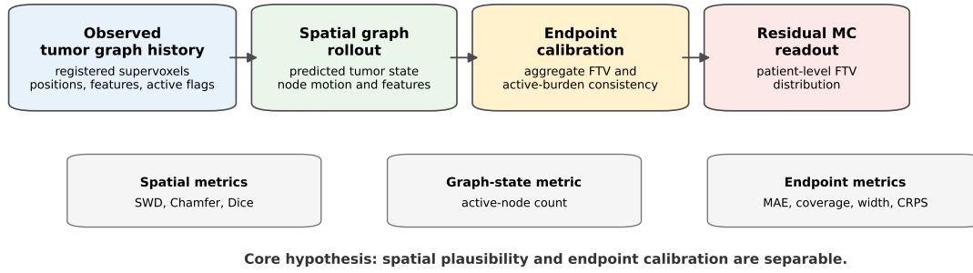
FIGURE 1. Endpoint-calibrated spatial forecasting separates the spatial tumor state from the endpoint and uncertainty layers queried from that state. The graph rollout is evaluated as a sampled tumor cloud and active-node state, while the FTV readout is evaluated with endpoint error, coverage, sharpness, and CRPS.
