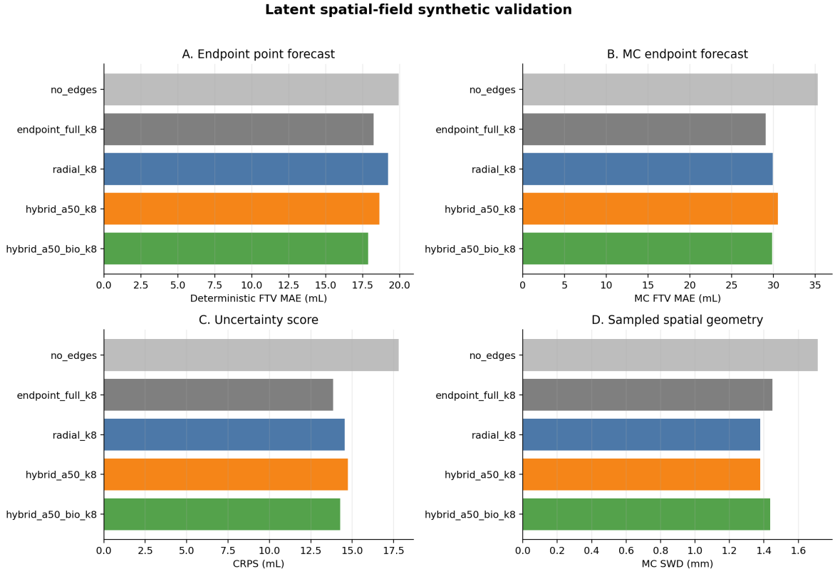
Fig. 2. Synthetic latent spatial-field validation. The retained graph becomes most useful when hidden regional response structure can be denoised through local neighborhoods, improving endpoint uncertainty and sampled-cloud geometry relative to the no-edge control.
