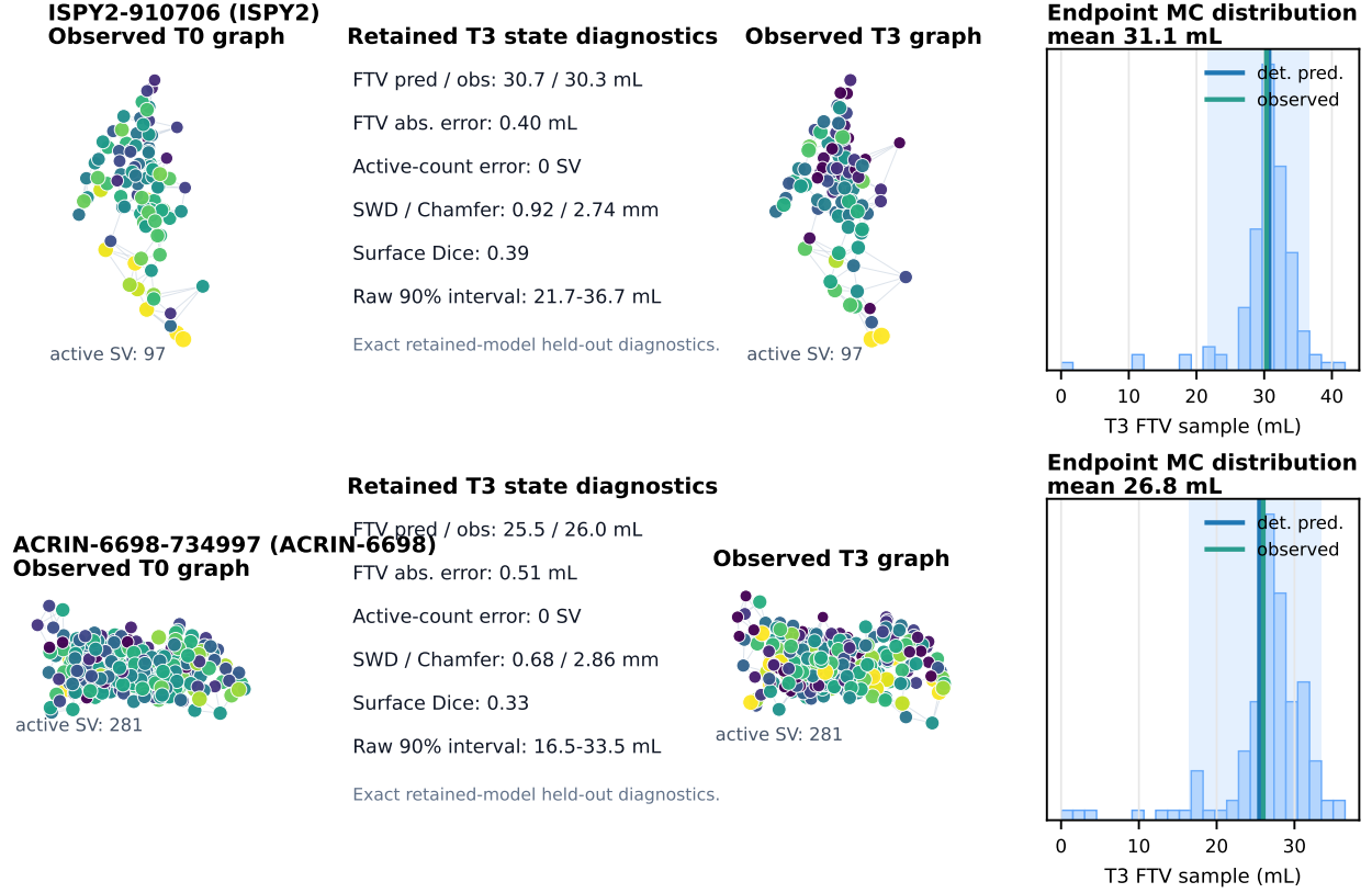
Fig. 3. Held-out graph-state and endpoint diagnostics from the retained HYBRID-EDGE k = 8 graph. Each row shows observed T_0 and T_3 active supervoxel graphs, exact retained-model T_3 graph-state diagnostics (FTV error, active-count error, SWD, Chamfer, and surface Dice), and the MC final-visit FTV distribution.
