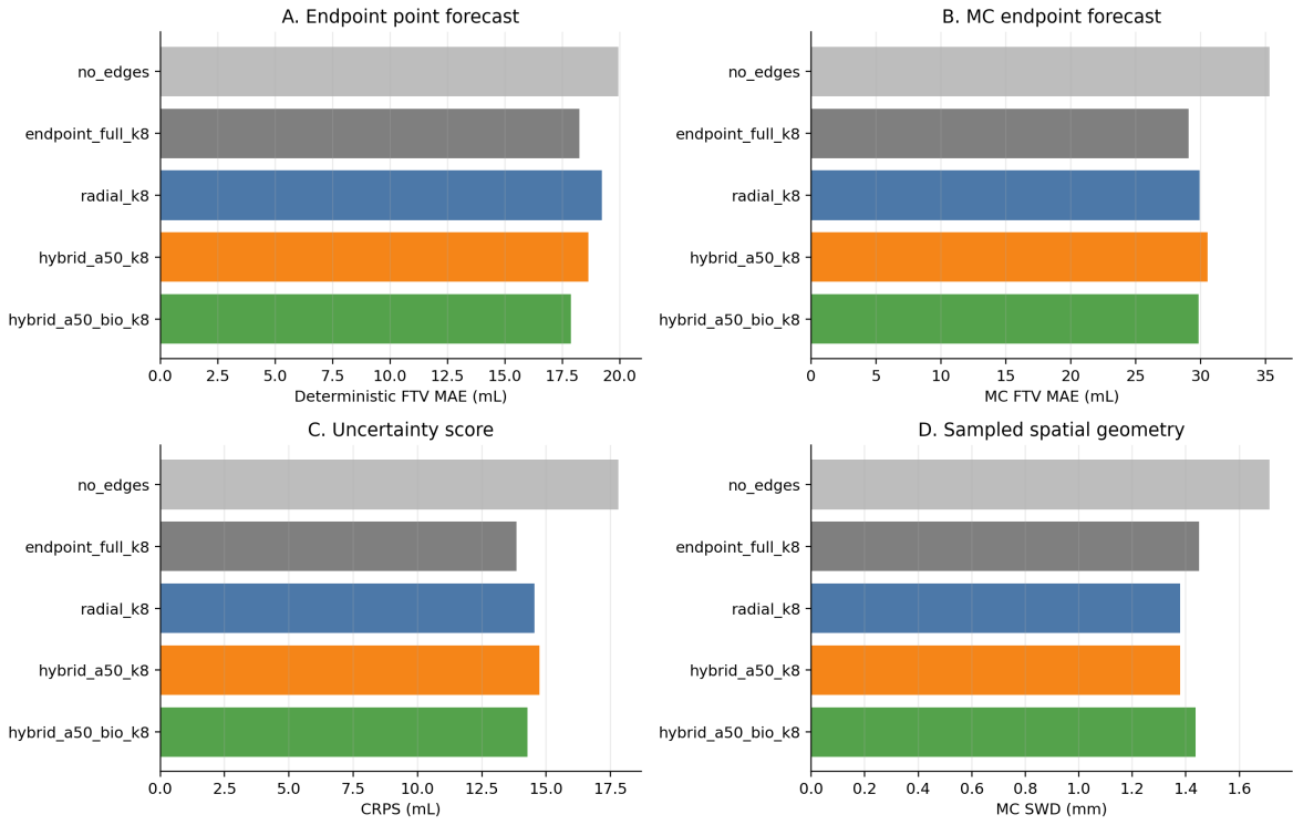
Fig. 2. Synthetic latent spatial-field validation. The retained graph becomes most useful when hidden regional response structure can be denoised through local neighborhoods, improving endpoint uncertainty and sampled-cloud geometry relative to the no-edge control.
