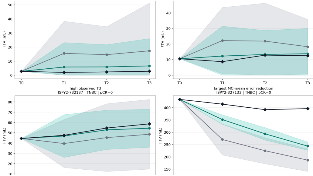
Figure 7: Representative T_0 \rightarrow T_3 Monte Carlo trajectory uncertainty examples. Gray shows the baseline MC mean and standard-deviation band, teal shows the retained-model MC mean and standard-deviation band, and black diamonds show observed FTV.
