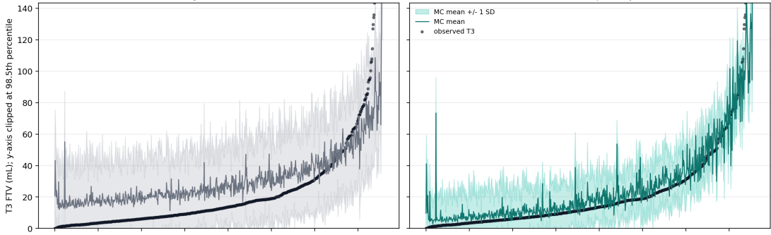
Figure 6: Cohort-wide T_0 \rightarrow T_3 MC uncertainty bands, with patients sorted by observed T_3 FTV. Endpoint calibration produces a narrower and better-centered patient-level distribution while improving raw coverage and CRPS.
