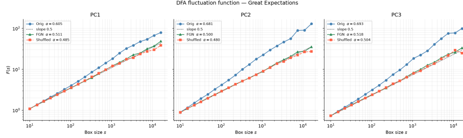
Figure 5: Log-log DFA fluctuation function F(s) for PC1, PC2, and PC3 — Great Expectations (Dickens). Each panel shows one component; the estimated exponent \alpha_k is given in the legend. Dotted line: reference slope 0.5. The original text (blue) has a consistently steeper slope than both null models, which are parallel to the \alpha = 0.5 reference across all box sizes s .
