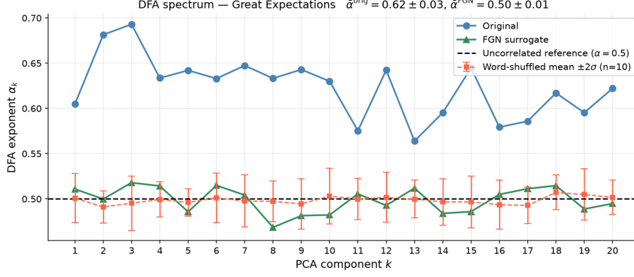
Figure 4: DFA scaling exponent \alpha_k of projected series x_t^{(k)} as a function of PCA component k — Great Expectations (Dickens). Blue circles: original filtered text. Green triangles: FGN surrogate. Red squares: word-shuffled null (mean \pm 2\sigma over 10 realisations). Dashed line: uncorrelated reference \alpha = 0.5 . The original text has \alpha_k > 0.5 for all 20 components; the FGN and shuffled are indistinguishable from \alpha = 0.5 .
