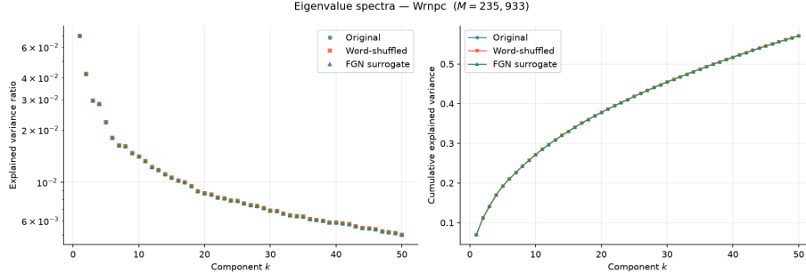
Figure 1: Eigenvalue spectra and cumulative explained variance for War and Peace . The three curves coincide: both surrogates are permutations of the original token sequence, so all three share the same covariance matrix and hence the same spectrum (Remark 2). The figure therefore verifies the construction rather than reporting a comparison.
