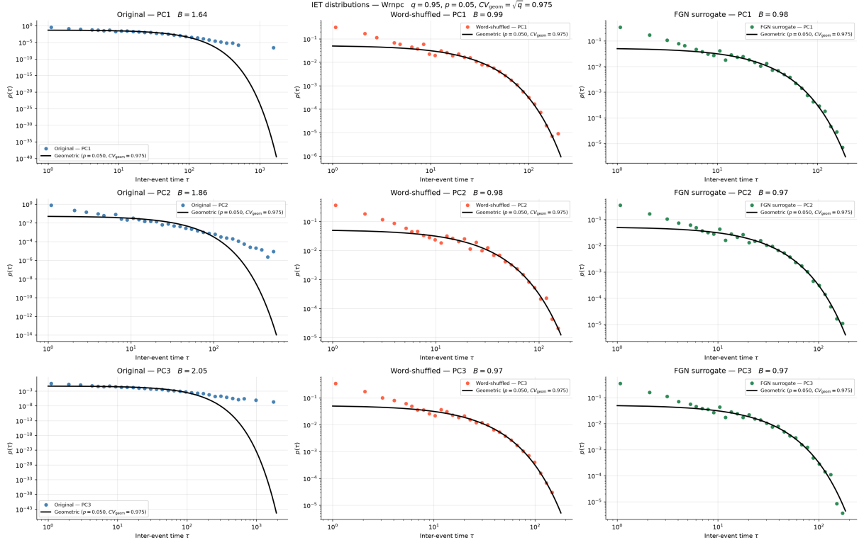
Figure 9: Inter-event-time distributions for PC1-PC3 of War and Peace at q = 0.95 . Columns show the original text (blue), word-shuffled null (red), and FGN surrogate (green). The original projections have broad tails, whereas both controls lie close to the geometric reference.
