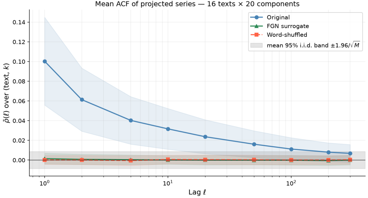
Figure 26: Mean ACF \bar{\rho}(\ell) of projected series across the corpus of 16 texts and K = 20 components, as a function of lag \ell (log scale). Shaded bands: \pm 1 standard deviation over (text, k ) pairs. Grey band: mean 95% i.i.d. confidence band \pm 1.96/\sqrt{M} . Blue circles: original filtered text. Green triangles: FGN surrogate. Red squares: word-shuffled null. The original maintains significant positive ACF across all lags tested ( \ell = 1, \dots, 300 ). Both null models are indistinguishable from zero at all lags.
