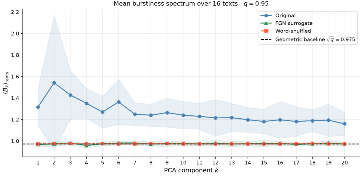
Figure 21: Mean component-resolved burstiness spectrum across the analysed corpus at q = 0.95 . Curves show the mean \langle B_k \rangle over texts for k = 1, \dots, 20 ; shaded bands indicate one standard deviation. The original texts (blue) are above the FGN surrogate (green), word-shuffled null (red), and geometric baseline \sqrt{q} \simeq 0.975 at every component. The largest corpus means occur among the early components, followed by a broad decline with non-monotone secondary peaks.
