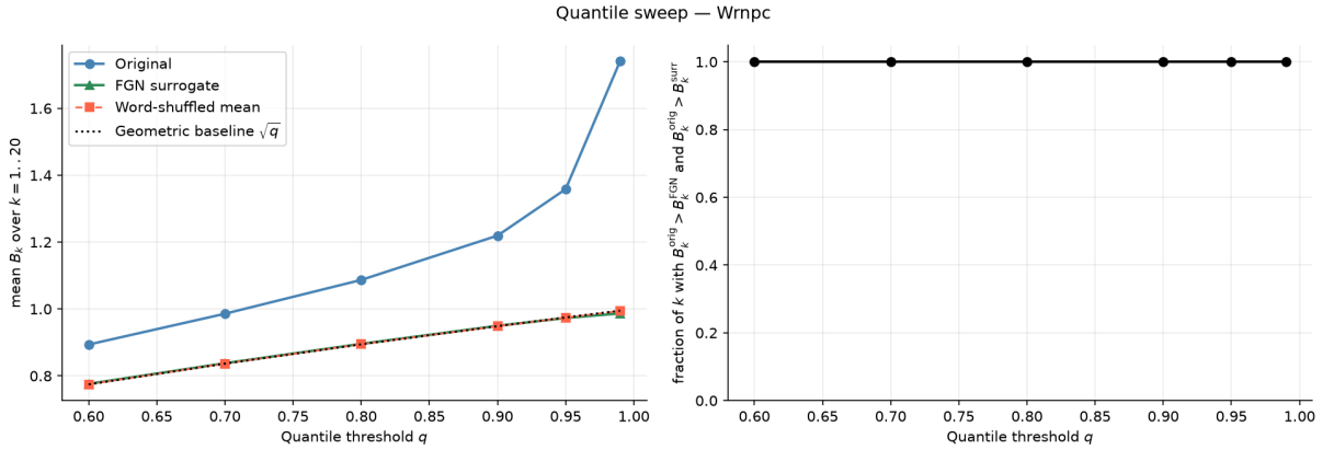
Figure 17: Quantile sweep for War and Peace . Left: mean B_k over k = 1, \dots, 20 as a function of q . Right: fraction of components satisfying the full ordering B_k^{\text{orig}} > B_k^{\text{FGN}} and B_k^{\text{orig}} > B_k^{\text{surr}} (100% across all q ).
