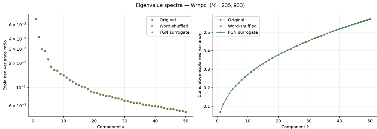
Figure 1: Eigenvalue spectra and cumulative explained variance for War and Peace : original (blue), word-shuffled (red), and FGN surrogate (green). The shuffled spectrum is identical to the original by permutation invariance; the FGN spectrum is empirically very close over the displayed range (Remark 2).
