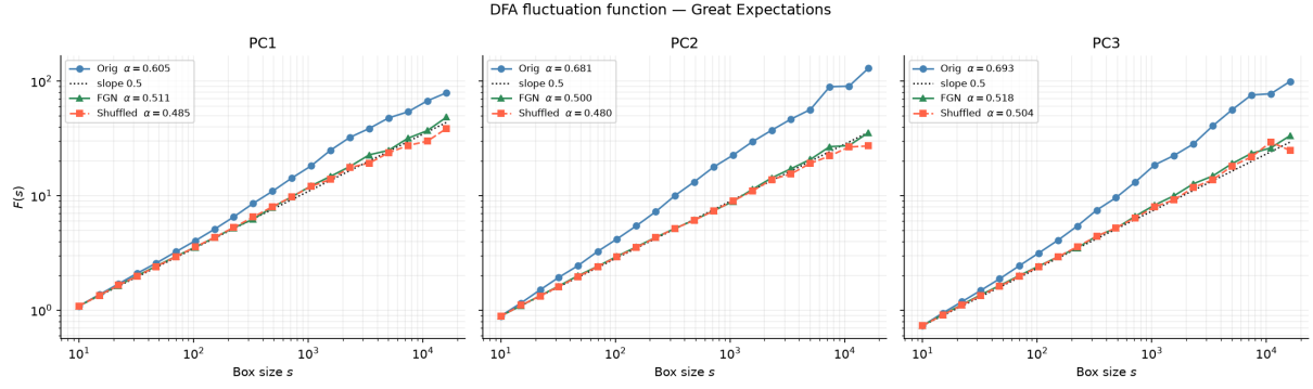
Figure 30: Log-log DFA fluctuation function F(s) for PC1, PC2, and PC3 — Great Expectations (Dickens). Each panel shows one component; the estimated exponent \alpha_k is given in the legend. Dotted line: reference slope 0.5. The original text (blue) has a consistently steeper slope than both null models, which are parallel to the \alpha = 0.5 reference across all box sizes s .
