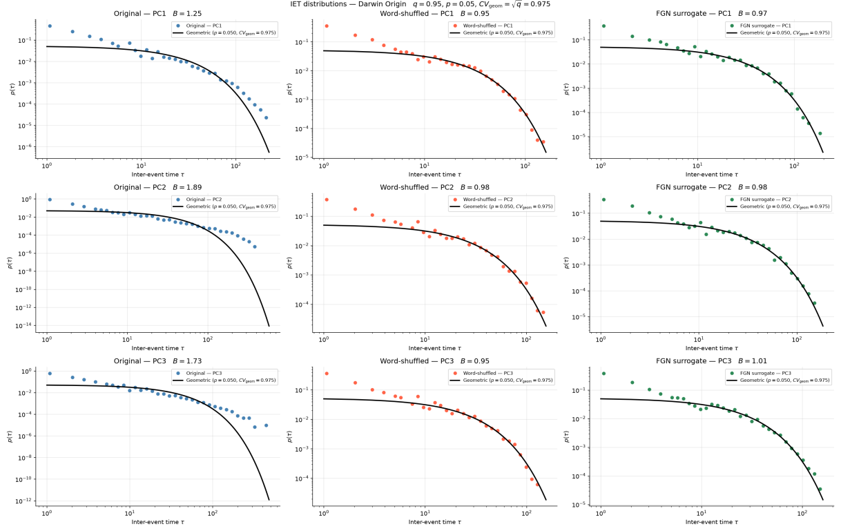
Figure 11: Inter-event time distributions for PC1, PC2, PC3 of On the Origin of Species ( q = 0.95 ). Same conventions as Figure 9.
