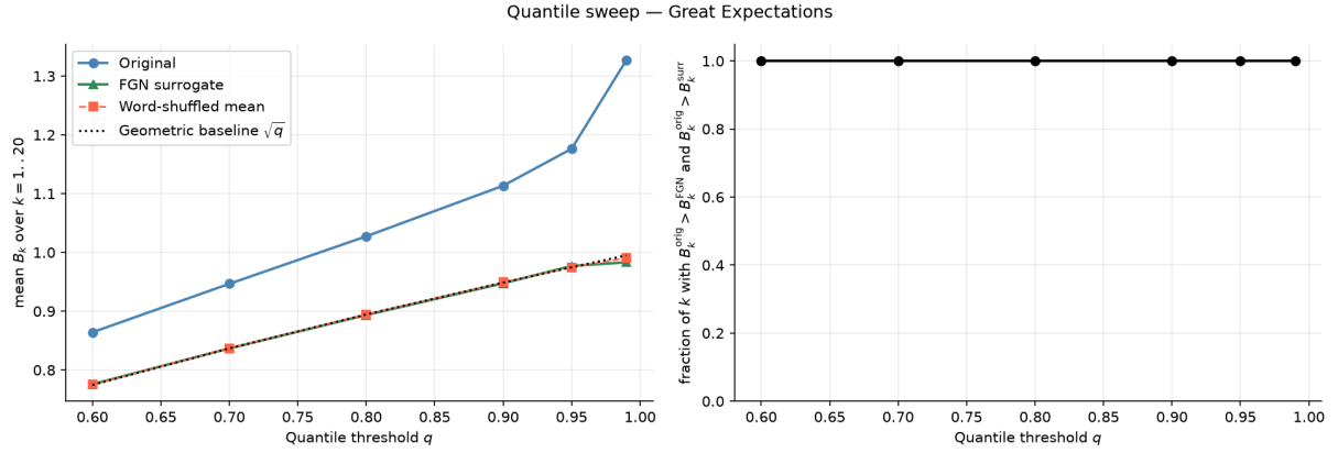
Figure 19: Quantile sweep for Great Expectations . Full ordering satisfied for 100% of components across all q \in [0.60, 0.99] .
