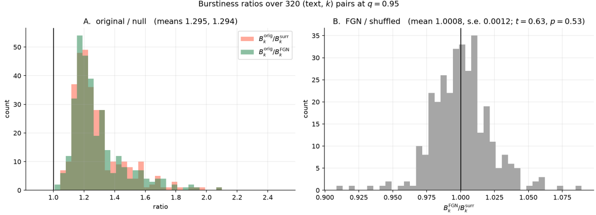
Figure 23: Distribution of burstiness ratios over 320 (text, k ) pairs at q = 0.95 . Panel A: distributions of B_k^{\text{orig}}/B_k^{\text{surr}} (red) and B_k^{\text{orig}}/B_k^{\text{FGN}} (green), both concentrated well above 1. The two distributions are nearly identical, confirming that the two null models are equivalently far below the original. Panel B: distribution of B_k^{\text{FGN}}/B_k^{\text{surr}} , tightly centred on 1 (mean 1.0008, s.e. 0.0012; t = 0.63, p = 0.53 ), statistically indistinguishable from unity, confirming B_k^{\text{FGN}} \approx B_k^{\text{surr}} across the entire corpus.
