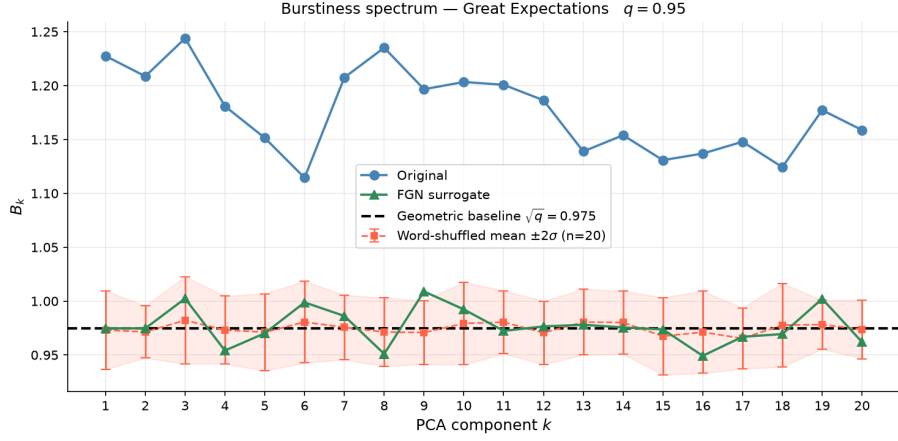
Figure 14: Component-resolved burstiness spectrum for Great Expectations at q = 0.95 . The original remains above both controls and the geometric baseline across all 20 components, with a comparatively flatter spectrum than in War and Peace .
