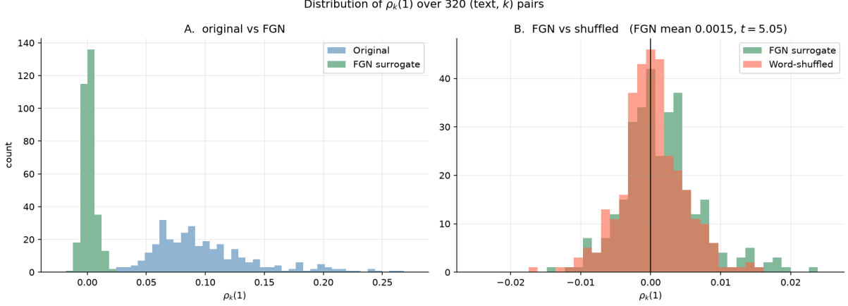
Figure 28: Distribution of \rho_k(1) over 320 (text, k ) pairs. Panel A: original (blue) and FGN (green). The two distributions are completely separated: all original pairs have \rho_k(1) > 0.007 (above the i.i.d. band), while nearly all FGN pairs are inside the band. Panel B: FGN (green) and word-shuffled (red) on an expanded scale. Both are centred near zero; a t -test gives t = 5.05 for \bar{\rho}^{\text{FGN}}(1) = 0 but the effect size is negligible (0.002) relative to the orig–null gap (0.098).
