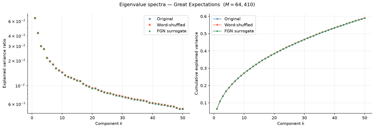
Figure 5: Eigenvalue spectra and cumulative explained variance for Great Expectations . Same conventions as Figure 1.
