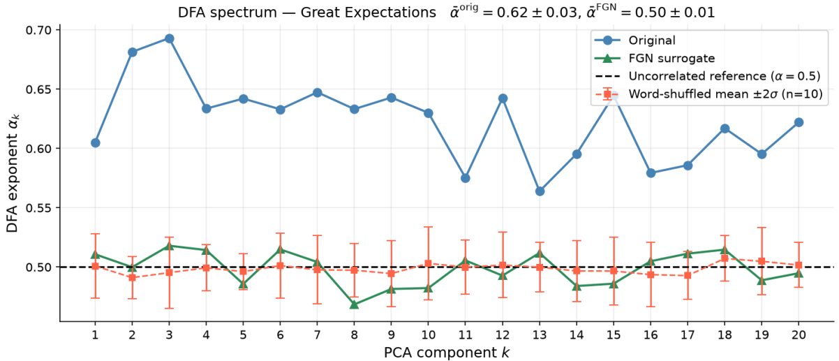
Figure 29: DFA scaling exponent \alpha_k of projected series x_t^{(k)} as a function of PCA component k — Great Expectations (Dickens). Blue circles: original filtered text. Green triangles: FGN surrogate. Red squares: word-shuffled null (mean \pm 2\sigma over 10 realisations). Dashed line: uncorrelated reference \alpha = 0.5 . The original text has \alpha_k > 0.5 for all 20 components; the FGN and shuffled are indistinguishable from \alpha = 0.5 .
