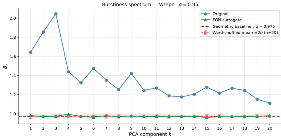
Figure 10: Component-resolved burstiness spectrum for War and Peace at q = 0.95 . The original (blue circles) is above the FGN surrogate (green triangles), the word-shuffled mean \pm 2\sigma band (red), and the geometric baseline \sqrt{q} \simeq 0.975 for all 20 components. Burstiness is largest among the first few components but is not monotone in PCA rank.
