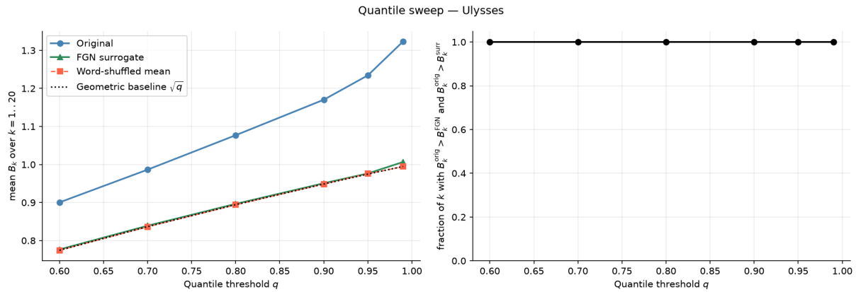
Figure 20: Quantile sweep for Ulysses . Full ordering satisfied for 100% of components across all q \in [0.60, 0.99] .
