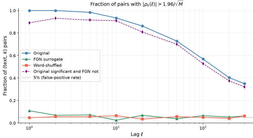
Figure 27: Fraction of text–component pairs with significant ACF as a function of lag \ell (log scale). Blue: original; green: FGN; red: word-shuffled; purple dashed: original significant and FGN not. The original remains clearly separated from both controls through lags of order 10^2 . The short-lag FGN excess is concentrated disproportionately in PC1, the component most affected by the embedding-geometry artefact discussed in Section 3.1.
