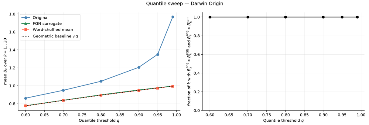
Figure 18: Quantile sweep for On the Origin of Species . Full ordering satisfied for 100% of components across all q \in [0.60, 0.99] .
