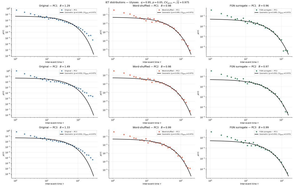
Figure 15: Inter-event time distributions for PC1, PC2, PC3 of Ulysses ( q = 0.95 ). Same conventions as Figure 9.
