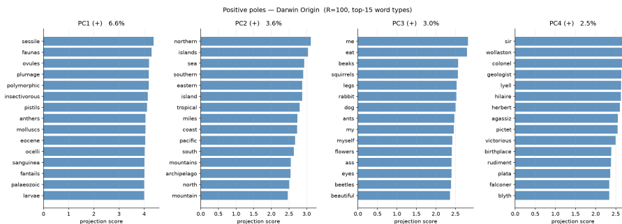
Figure 4: Positive poles of PC1–PC4 for On the Origin of Species . PC2 separates geographical distribution chapters from theoretical reasoning chapters; PC3 separates field-observation passages from abstract synthesis.
