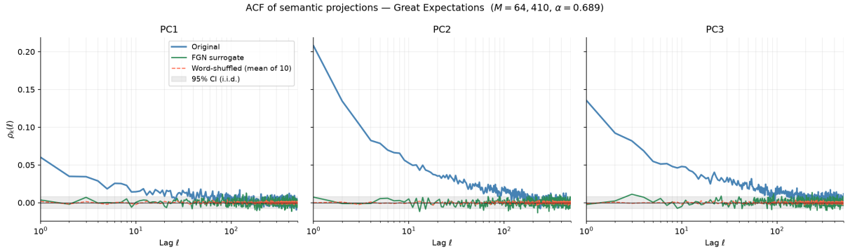
Figure 24: Autocorrelation function \rho_k(\ell) of projected series, as a function of lag \ell (log scale) — Great Expectations (Dickens). Each panel shows one PCA component (PC1, PC2, PC3). Blue: original filtered text. Green: FGN surrogate. Red dashed: word-shuffled null (mean over 10 realisations). Grey band: \pm 1.96/\sqrt{M} i.i.d. reference (95% CI). The original text has substantial positive ACF that decays slowly on a log scale, remaining above the i.i.d. band up to \ell \sim 100 . Both null models collapse immediately into the i.i.d. band, despite the FGN surrogate having the same DFA exponent \alpha = 0.689 as the original.
