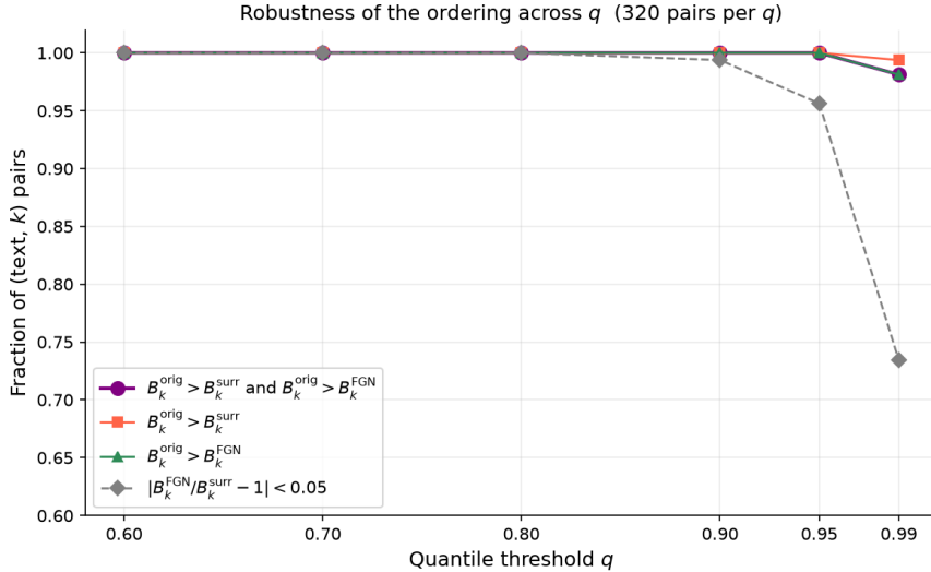
Figure 22: Robustness of the burstiness ordering across quantile threshold q . Each point: fraction of (text, k ) pairs (320 per q ) satisfying the indicated condition. Purple circles: full ordering B_k^{\text{orig}} > B_k^{\text{surr}} and B_k^{\text{orig}} > B_k^{\text{FGN}} . Red squares: B_k^{\text{orig}} > B_k^{\text{surr}} . Green triangles: B_k^{\text{orig}} > B_k^{\text{FGN}} . Grey diamonds: |B_k^{\text{FGN}}/B_k^{\text{surr}} - 1| < 0.05 . The ordering is robust for q \in [0.60, 0.95] ; the slight degradation at q = 0.99 is due to estimator noise at p = 0.01 .
