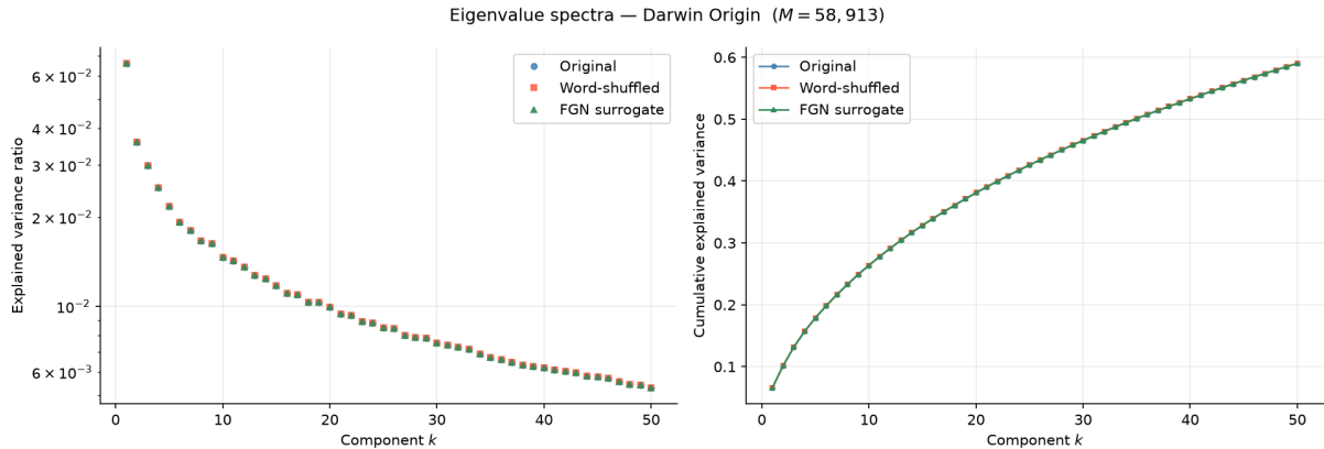
Figure 3: Eigenvalue spectra and cumulative explained variance for On the Origin of Species . Same conventions as Figure 1.
