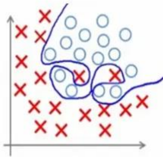
Over-fitting
