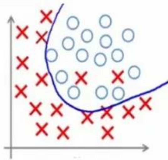
Appropriate-fitting
