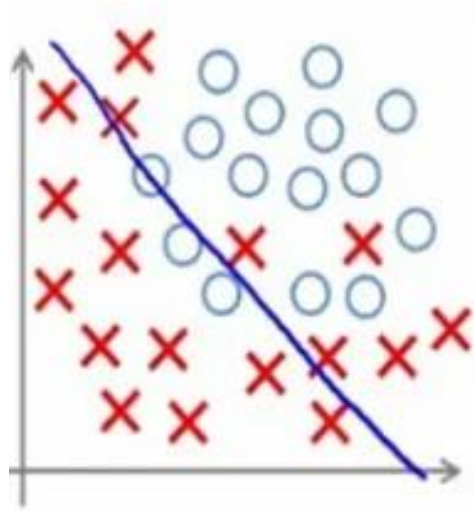
Under-fitting
