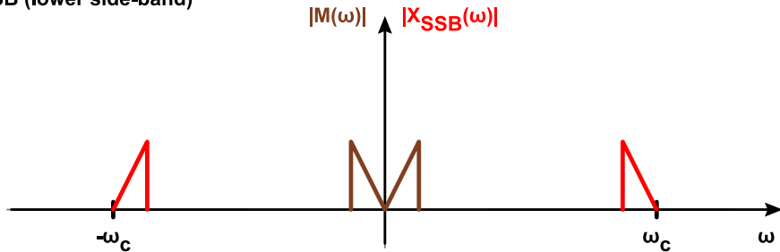
SSB (lower side-band)
