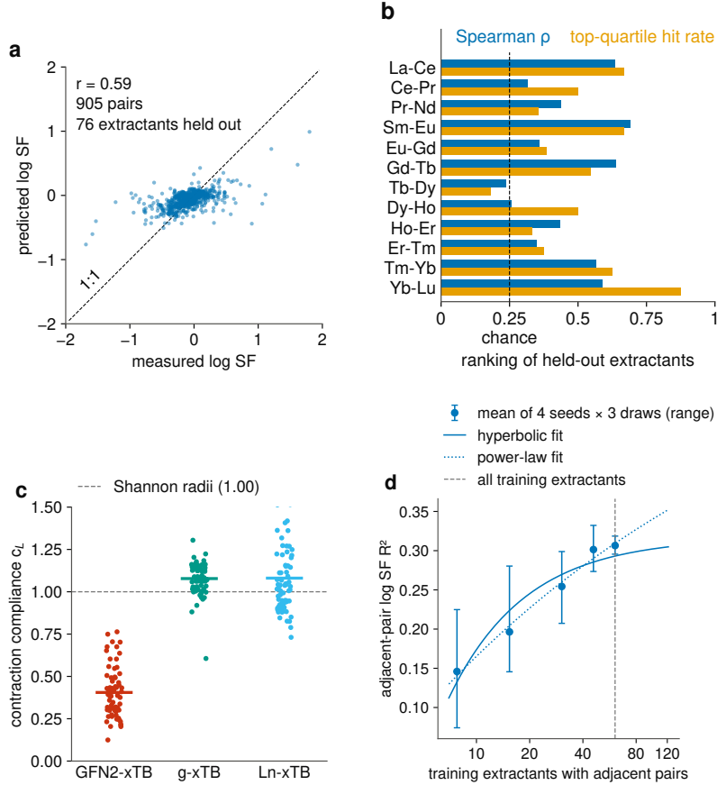
Figure 1: (a) Predicted against measured adjacent-pair log SF for the 905 development pairs, extractants held out; the dashed line is the identity. (b) Per adjacent pair: Spearman \rho between predicted and measured extractant rankings, and the top-quartile hit rate against chance. (c) Contraction compliance c_L of 71 ligands under three Hamiltonians; 1.00 is exact agreement with the Shannon radii. (d) Learning curve over training extractants (four CV seeds, three nested draws; whiskers span the runs; hyperbolic and power-law extrapolations; dashed line, full training set).
