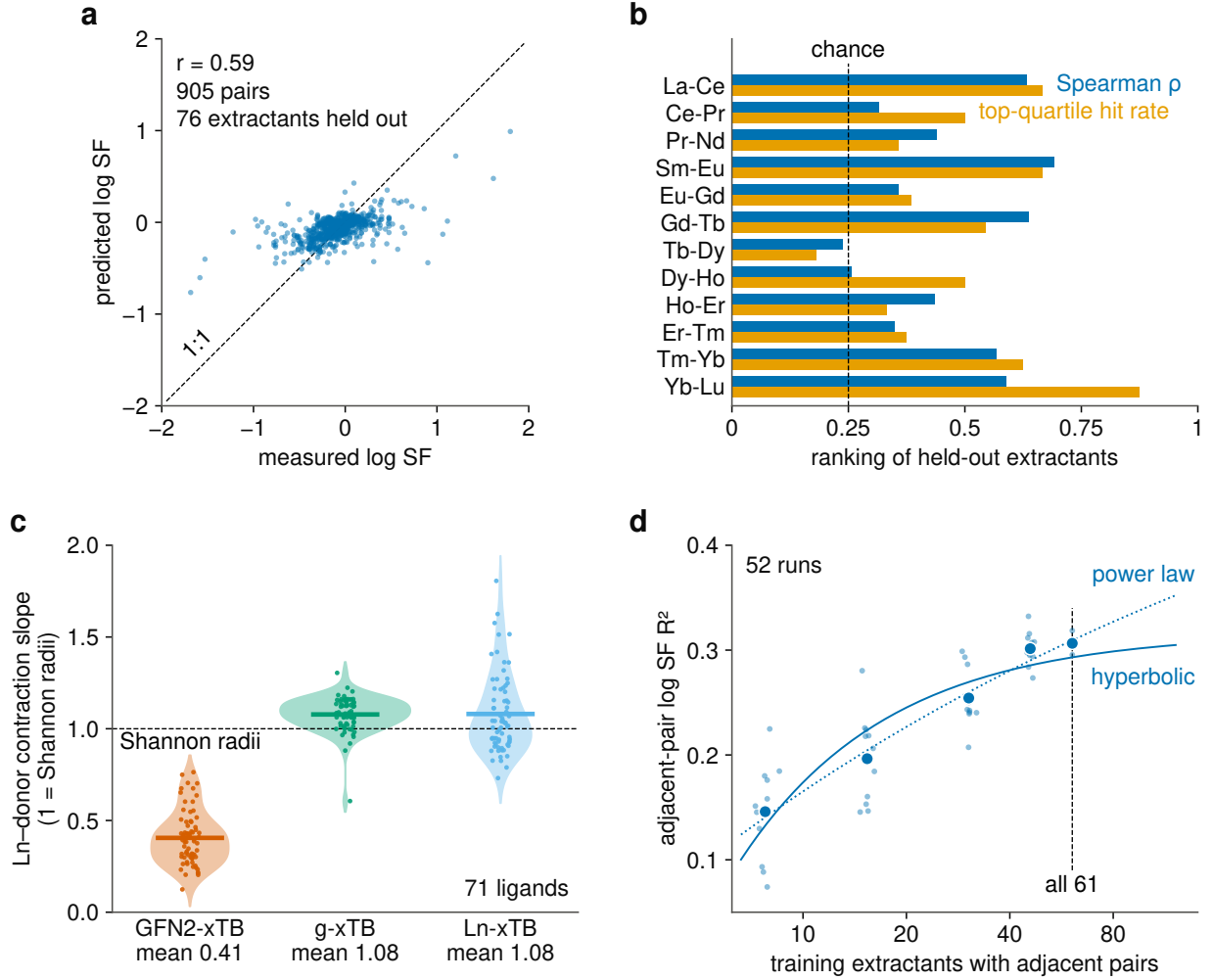
Figure 1: (a) Predicted against measured adjacent-pair logSF for the 905 development pairs, extractants held out; the dashed line is the identity. (b) Per adjacent pair: Spearman \rho between predicted and measured extractant rankings, and the top-quartile hit rate against chance. (c) Slope of the Ln-donor distance against the Shannon radius (the compliance c_L ) for the 71 ligands under three Hamiltonians: points are ligands, shaded shapes their kernel density, bars the mean; 1 is exact agreement with the radii. (d) Learning curve: small points are the 52 individual runs (four CV seeds, three nested draws) at their own training size, large markers the mean per fraction; solid and dotted lines the hyperbolic and power-law extrapolations; dashed line the full training set.
