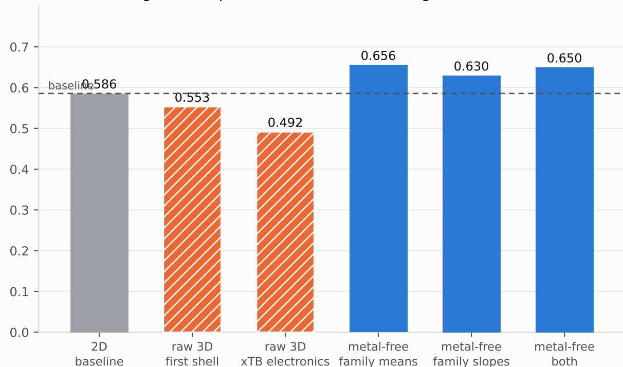
series ordering: mean Spearman across La→Lu (higher = better)
