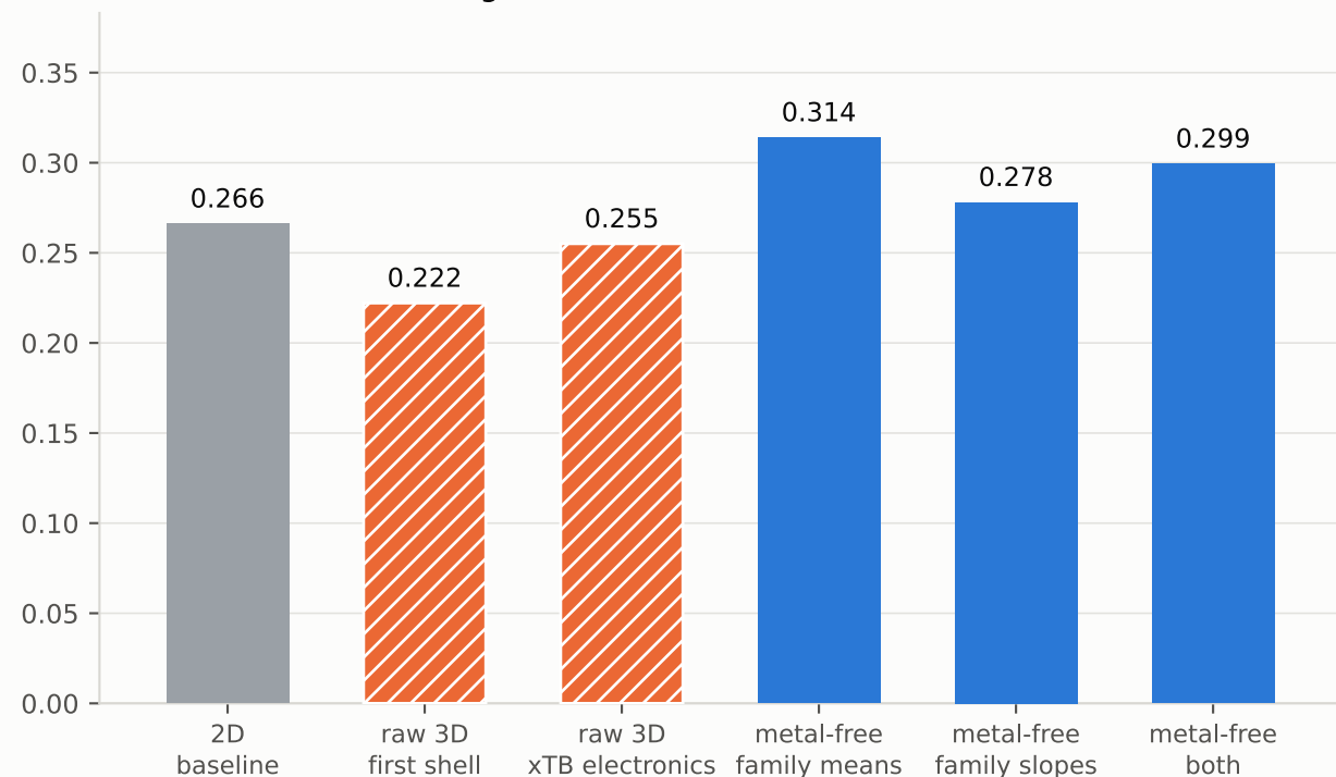
R^2 within extractant (higher = better)
