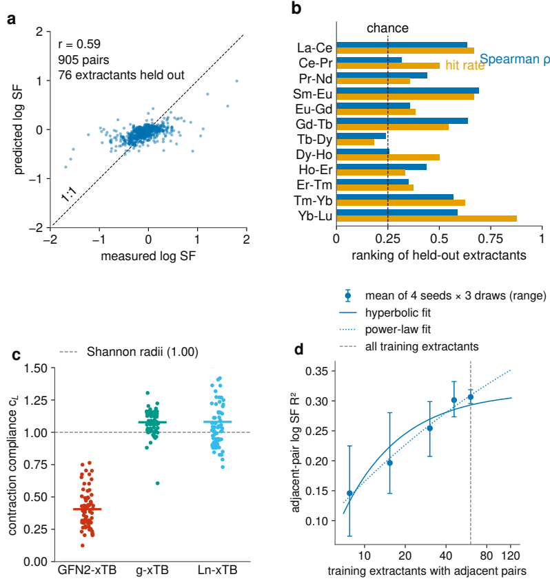
Figure 1: (a) Predicted against measured adjacent-pair logSF for the 905 development pairs, extractants held out; the dashed line is the identity. (b) Per adjacent pair: Spearman \rho between predicted and measured extractant rankings, and the top-quartile hit rate against chance. (c) Contraction compliance c_L of 71 ligands under three Hamiltonians; 1.00 is exact agreement with the Shannon radii. (d) Learning curve over training extractants (four CV seeds, three nested draws; whiskers span the runs; hyperbolic and power-law extrapolations; dashed line, full training set).
