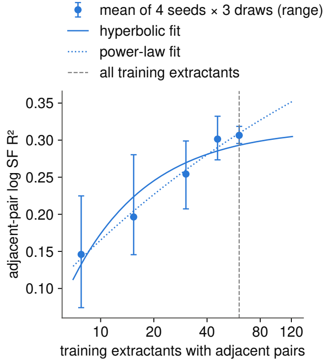
Figure 4: Adjacent-pair R^2 on the 905 legacy pairs when the level/shape model is trained on a random fraction of each fold’s training extractants (nested draws, four CV seeds, three draws each; whiskers span the runs). The two lines are the fitted extrapolations, hyperbolic (solid) and power law (dotted), which bracket the gain from doubling the extractants at +0.01 to +0.04; the dashed line marks the full training set.
