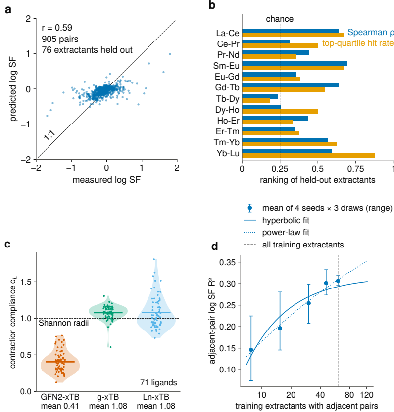
Figure 1: (a) Predicted against measured adjacent-pair log SF for the 905 development pairs, extractants held out; the dashed line is the identity. (b) Per adjacent pair: Spearman \rho between predicted and measured extractant rankings, and the top-quartile hit rate against chance. (c) Contraction compliance c_L of the 71 ligands under three Hamiltonians: points are ligands, shaded shapes their kernel density, bars the mean; 1.00 is exact agreement with the Shannon radii. (d) Learning curve over training extractants (four CV seeds, three nested draws; whiskers span the runs; hyperbolic and power-law extrapolations; dashed line, full training set).
