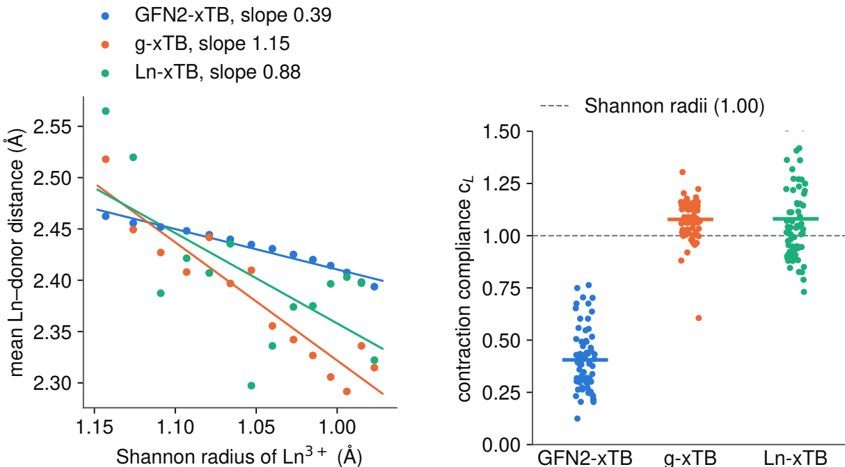
Figure 3: The lanthanide contraction in 71 ligand complexes. Left: one ligand (the one at GFN2-xTB’s median compliance), mean Ln-donor distance against the Shannon radius across Ce–Lu under the three Hamiltonians, with the fitted slopes. Right: the per-ligand compliance c_L for all 71 ligands, with the mean of each Hamiltonian as a bar; 1.00 is exact agreement with the ionic radii.
