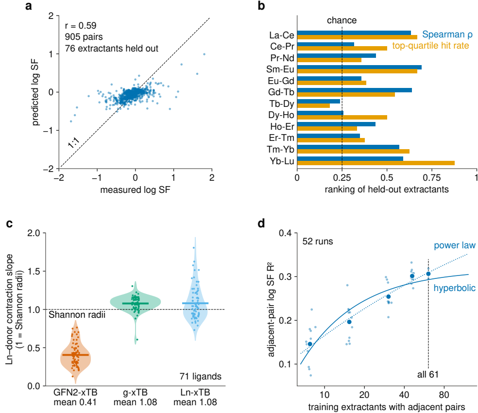
Figure 1: (a) Predicted against measured adjacent-pair log SF for the 905 development pairs, extractants held out; the dashed line is the identity. (b) Per adjacent pair: Spearman \rho between predicted and measured extractant rankings, and the top-quartile hit rate against chance. (c) Slope of the Ln-donor distance against the Shannon radius (the compliance c_L ) for the 71 ligands under three Hamiltonians: points are ligands, shaded shapes their kernel density, bars the mean; 1 is exact agreement with the radii. (d) Learning curve: small points are the 52 individual runs (four CV seeds, three nested draws) at their own training size, large markers the mean per fraction; solid and dotted lines the hyperbolic and power-law extrapolations; dashed line the full training set.
