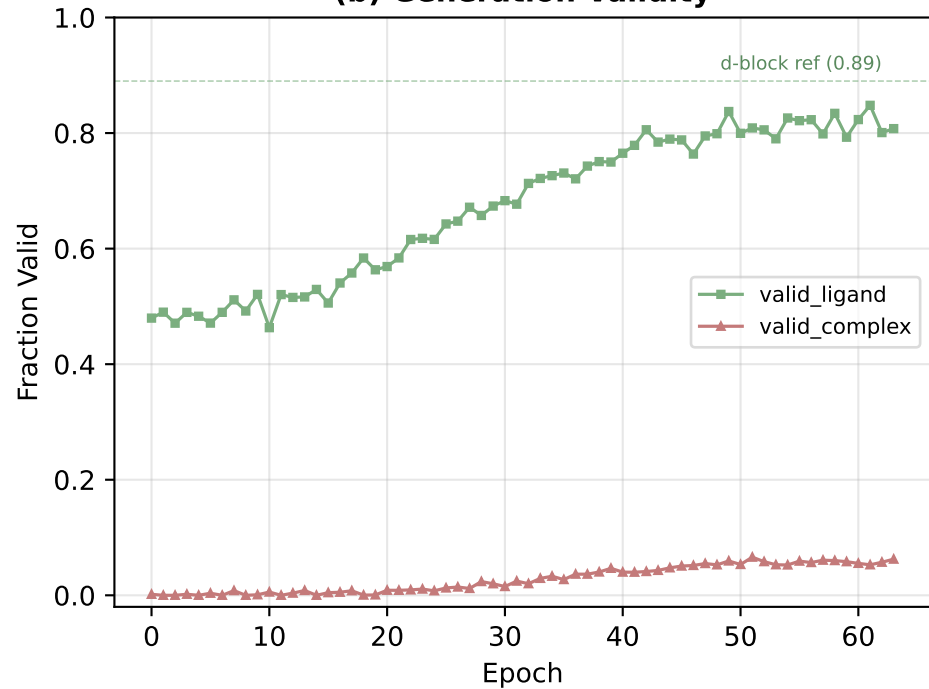
(b) Generation Validity
