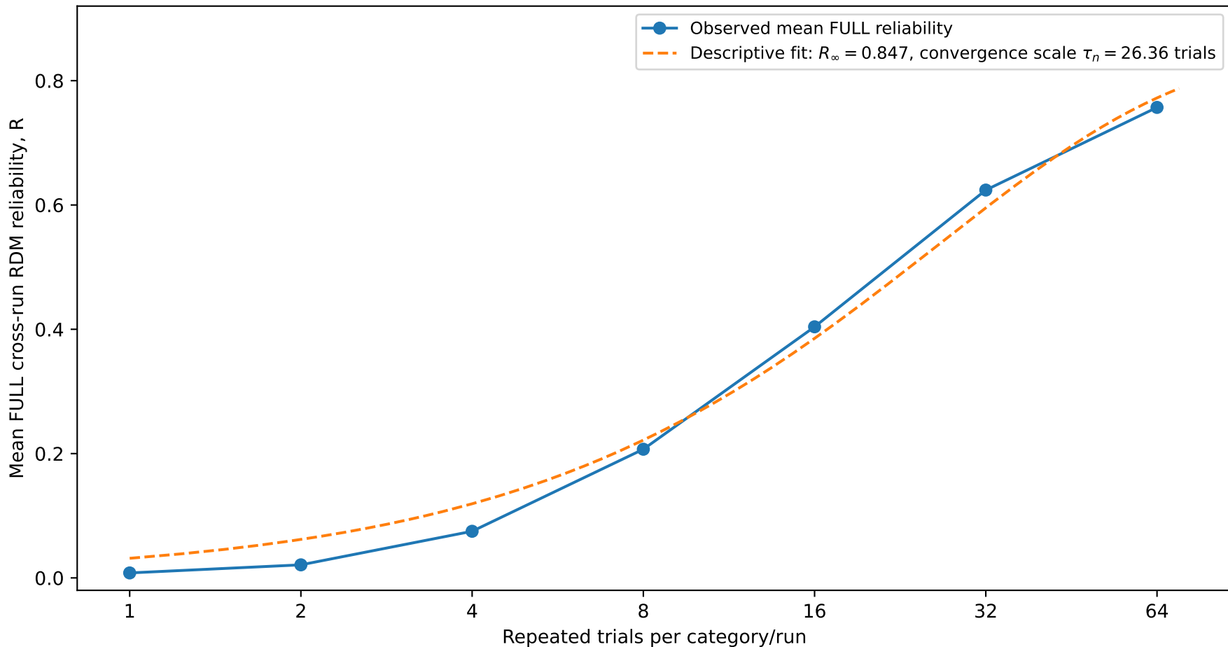
Ensemble reliability increases with repeated-trial averaging (descriptive, not prescriptive)
