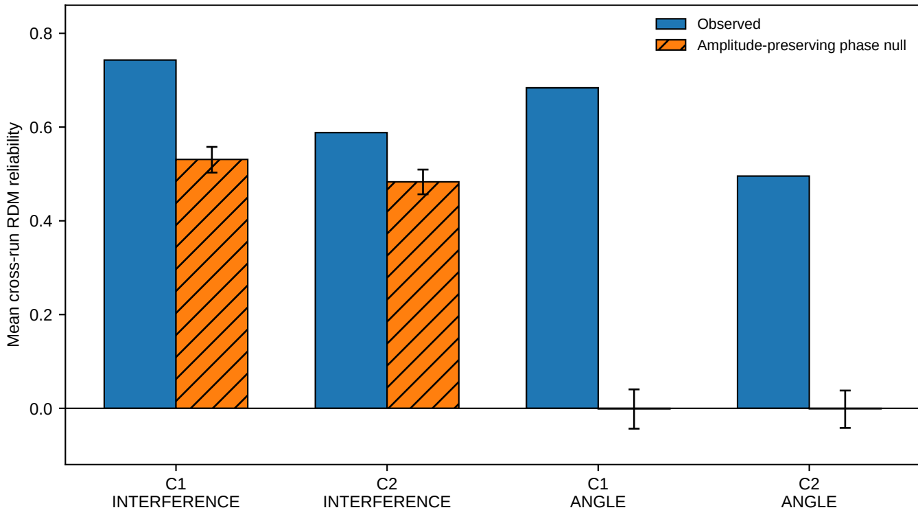
Category-specific phase organization exceeds amplitude-preserving nulls
