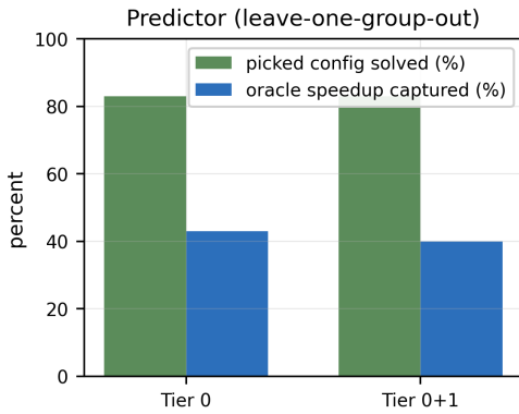
Fig. 4. Predictor under leave-one-group-out: fraction of held-out matrices whose picked configuration solves, and fraction of oracle speedup captured. Tier 0 (near-free) matches Tier 0+1.
