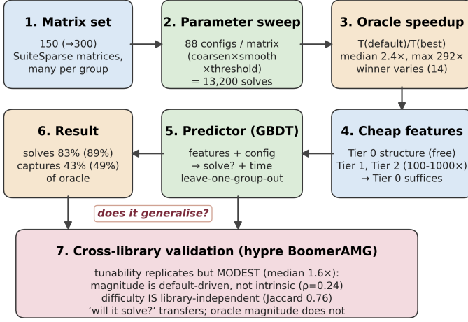
Fig. 1. Overview. We sweep 88 internal configurations of AMGCL over 150 (later 300) SuiteSparse matrices (1–2), measure the per-matrix oracle speedup of the best configuration over the default (3), and train a predictor on cheap matrix features to pick a good configuration under a leave-one-group-out protocol (4–6). We then repeat the sweep on HYPRE BoomerAMG to test whether the findings generalise (7): tunability replicates but its magnitude is default-driven and does not transfer between libraries, whereas intrinsic solvability does.
