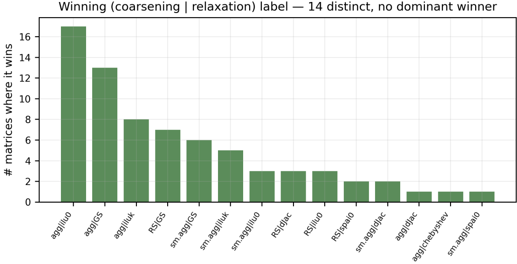
Fig. 3. Frequency with which each (coarsening | relaxation) label is the per-matrix winner. The spread across 14 labels shows that per-matrix selection, not a single improved default, is what the speedup requires.
