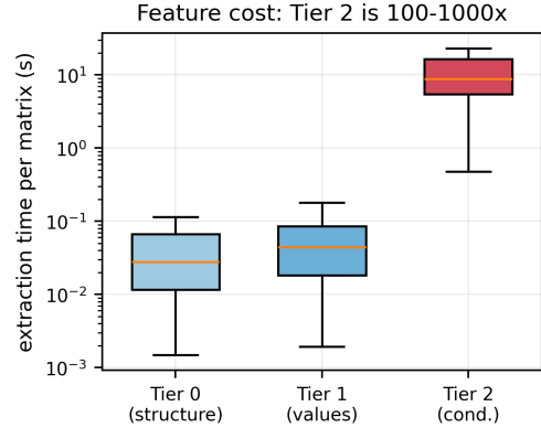
Fig. 5. Feature-extraction time per matrix by tier (log scale). Tier 2 costs 100–1000× Tier 0/1 yet buys no predictive accuracy here.
