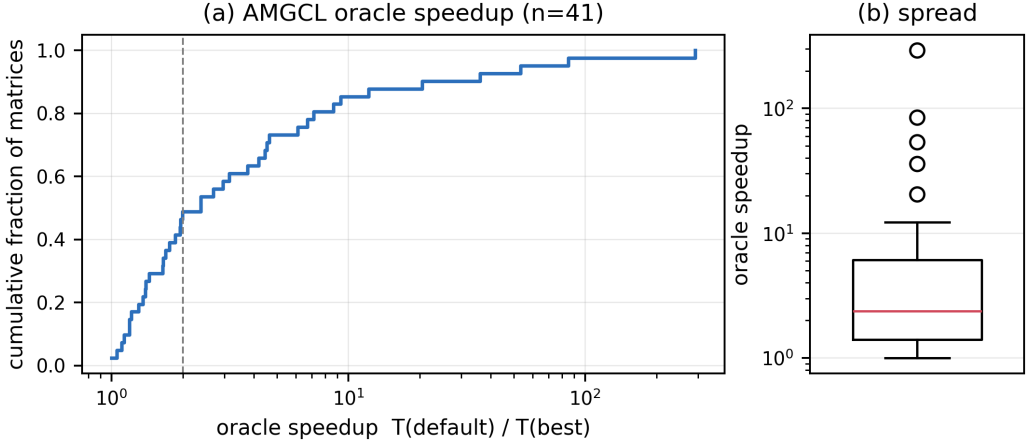
Fig. 2. AMGCL oracle speedup over 41 matrices: (a) empirical CDF (log axis; dashed line at 2 \times ), (b) distribution on a log scale. Median 2.4 \times , upper quartile 6.4 \times , maximum 292 \times .
