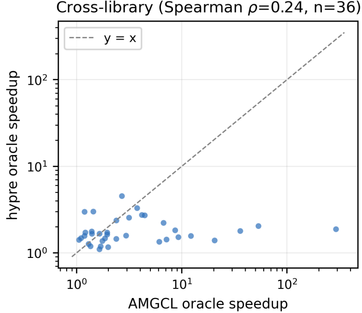
Figure 6: Per-matrix oracle speedup: AMGCL vs HYPRE (both log axes, n = 36 ). The weak rank correlation ( \rho = 0.24 ) shows tuning benefit does not transfer between libraries; the largest AMGCL gains are where HYPRE’s default already wins.
