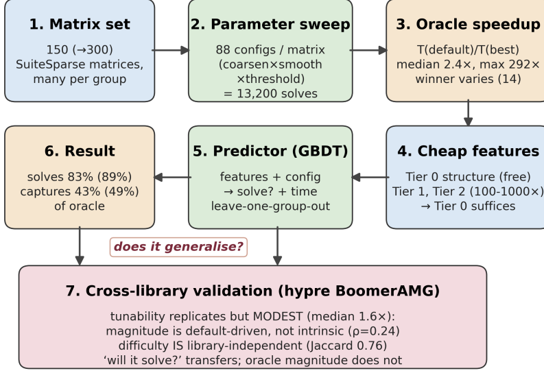
Figure 1: Overview. We sweep 88 internal configurations of AMGCL over 150 (later 300) SuiteSparse matrices (1–2), measure the per-matrix oracle speedup of the best configuration over the default (3), and train a predictor on cheap matrix features to pick a good configuration under a leave-one-group-out protocol (4–6). We then repeat the sweep on HYPRE BoomerAMG to test whether the findings generalise (7): tunability replicates but its magnitude is default-driven and does not transfer between libraries, whereas intrinsic solvability does.
