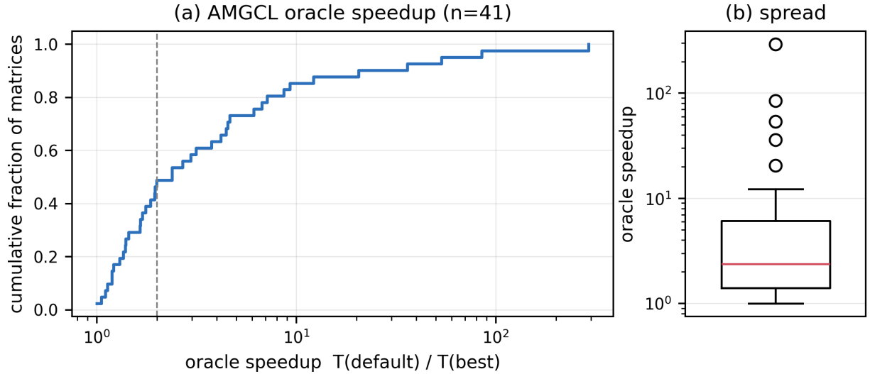
Figure 2: AMGCL oracle speedup over 41 matrices: (a) empirical CDF (log axis; dashed line at 2\times ), (b) distribution on a log scale. Median 2.4\times , upper quartile 6.4\times , maximum 292\times .
