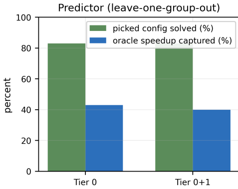
Fig. 3. Predictor under leave-one-group-out: fraction of held-out matrices whose picked configuration solves, and fraction of oracle speedup captured. Tier 0 (near-free) matches Tier 0+1.
