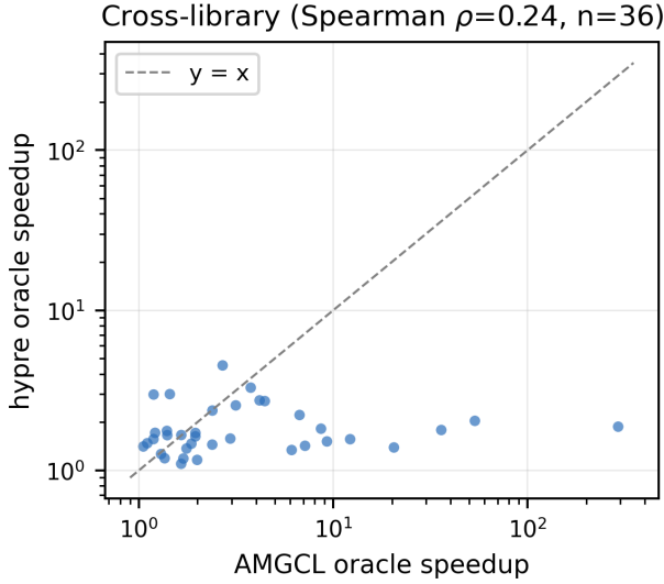
Fig. 5. Per-matrix oracle speedup: AMGCL vs HYPRE (both log axes, n = 36 ). The weak rank correlation ( \rho = 0.24 ) shows tuning benefit does not transfer between libraries; the largest AMGCL gains are where HYPRE's default already wins.
