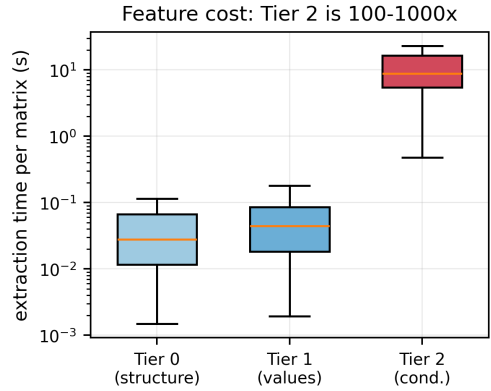
Fig. 4. Feature-extraction time per matrix by tier (log scale). Tier 2 costs 100–1000× Tier 0/1 yet buys no predictive accuracy here.
