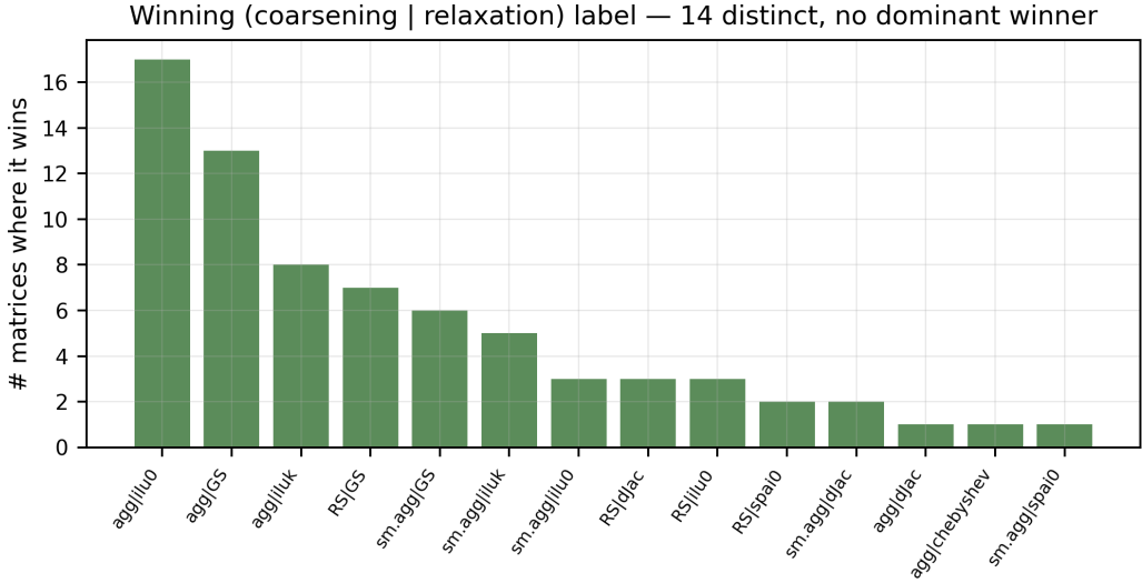
Fig. 2. Frequency with which each (coarsening | relaxation) label is the per-matrix winner. The spread across 14 labels shows that per-matrix selection, not a single improved default, is what the speedup requires.
