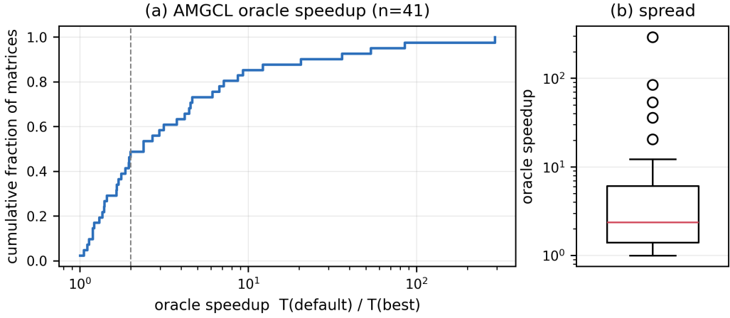
Fig. 1. AMGCL oracle speedup over 41 matrices: (a) empirical CDF (log axis; dashed line at 2 \times ), (b) distribution on a log scale. Median 2.4 \times , upper quartile 6.4 \times , maximum 292 \times .
