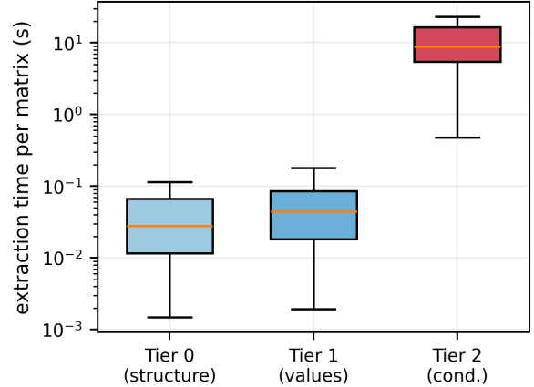
Figure 5: Feature-extraction time per matrix by tier (log scale). Tier 2 costs 100–1000 \times Tier 0/1 yet buys no predictive accuracy here.
