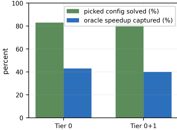
Figure 4: Predictor under leave-one-group-out: fraction of held-out matrices whose picked configuration solves, and fraction of oracle speedup captured. Tier 0 (near-free) matches Tier 0+1.
