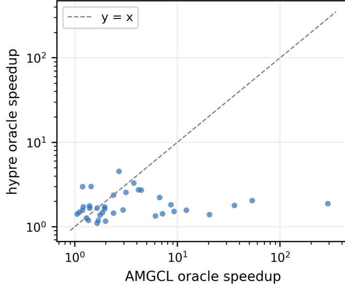
Figure 6: Per-matrix oracle speedup: AMGCL vs HYPRE (both log axes, n = 36 ). The weak rank correlation ( \rho = 0.24 ) shows tuning benefit does not transfer between libraries; the largest AMGCL gains are where HYPRE’s default already wins.
