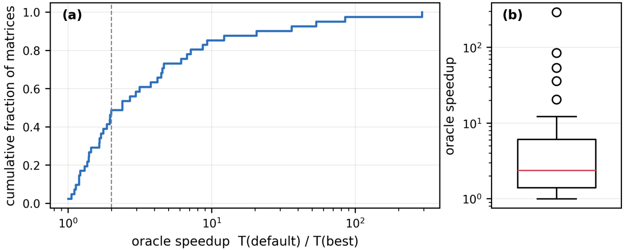
Figure 2: AMGCL oracle speedup over 41 matrices: (a) empirical CDF (log axis; dashed line at 2\times ), (b) distribution on a log scale. Median 2.4\times , upper quartile 6.4\times , maximum 292\times .
