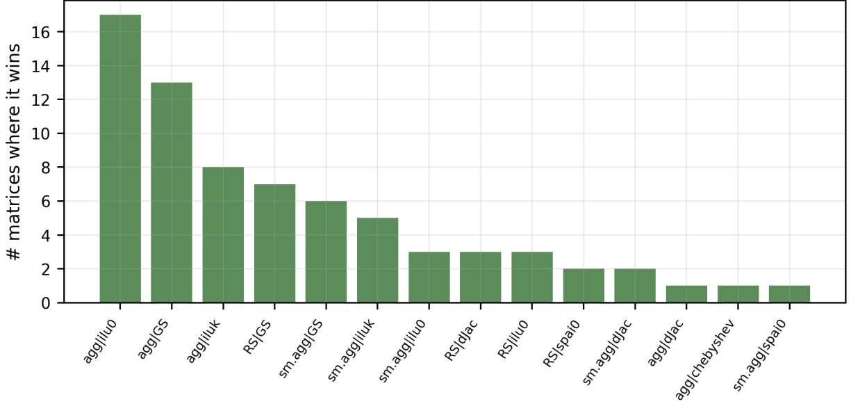
Figure 3: Frequency with which each (coarsening | relaxation) label is the per-matrix winner. The spread across 14 labels shows that per-matrix selection, not a single improved default, is what the speedup requires.
