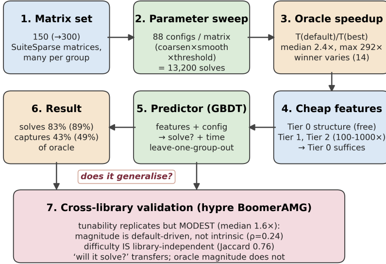
Fig. 1. Overview of the study, which asks three questions about tuning the internal parameters of AMG: how much is there to gain, can a good configuration be predicted, and does it generalise? We sweep 88 internal configurations of AMGCL over 150 (later 300) SuiteSparse matrices (1–2), measure the per-matrix oracle speedup of the best configuration over the default (3), and train a predictor on cheap matrix features to pick a good configuration under a leave-one-group-out protocol (4–6). We then repeat the sweep on HYPRE BoomerAMG to test whether the findings generalise (7): tunability replicates but its magnitude is default-driven and does not transfer between libraries, whereas intrinsic solvability does.
