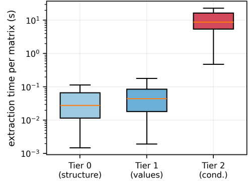
Fig. 5. Feature-extraction time per matrix by tier (log scale). Tier 2 costs 100–1000× Tier 0/1 yet buys no predictive accuracy here.
