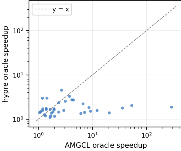
Fig. 6. Per-matrix oracle speedup: AMGCL vs HYPRE (both log axes, n = 36 ). The weak rank correlation ( \rho = 0.24 ) shows tuning benefit does not transfer between libraries; the largest AMGCL gains are where HYPRE's default already wins.
