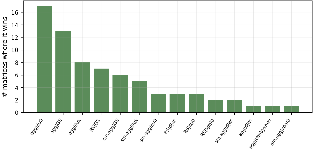
Fig. 3. Frequency with which each (coarsening | relaxation) label is the per-matrix winner. The spread across 14 labels shows that per-matrix selection, not a single improved default, is what the speedup requires.
