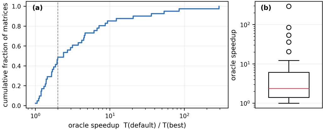
Fig. 2. AMGCL oracle speedup over 41 matrices: (a) empirical CDF (log axis; dashed line at 2 \times ), (b) distribution on a log scale. Median 2.4 \times , upper quartile 6.4 \times , maximum 292 \times .
