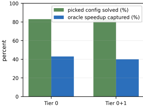
Fig. 4. Predictor under leave-one-group-out: fraction of held-out matrices whose picked configuration solves, and fraction of oracle speedup captured. Tier 0 (near-free) matches Tier 0+1.
