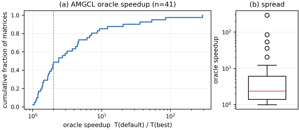
Fig. 1. AMGCL oracle speedup over 41 matrices: (a) empirical CDF (log axis; dashed line at 2\times ), (b) distribution on a log scale. Median 2.4\times , upper quartile 6.4\times , maximum 292\times .
