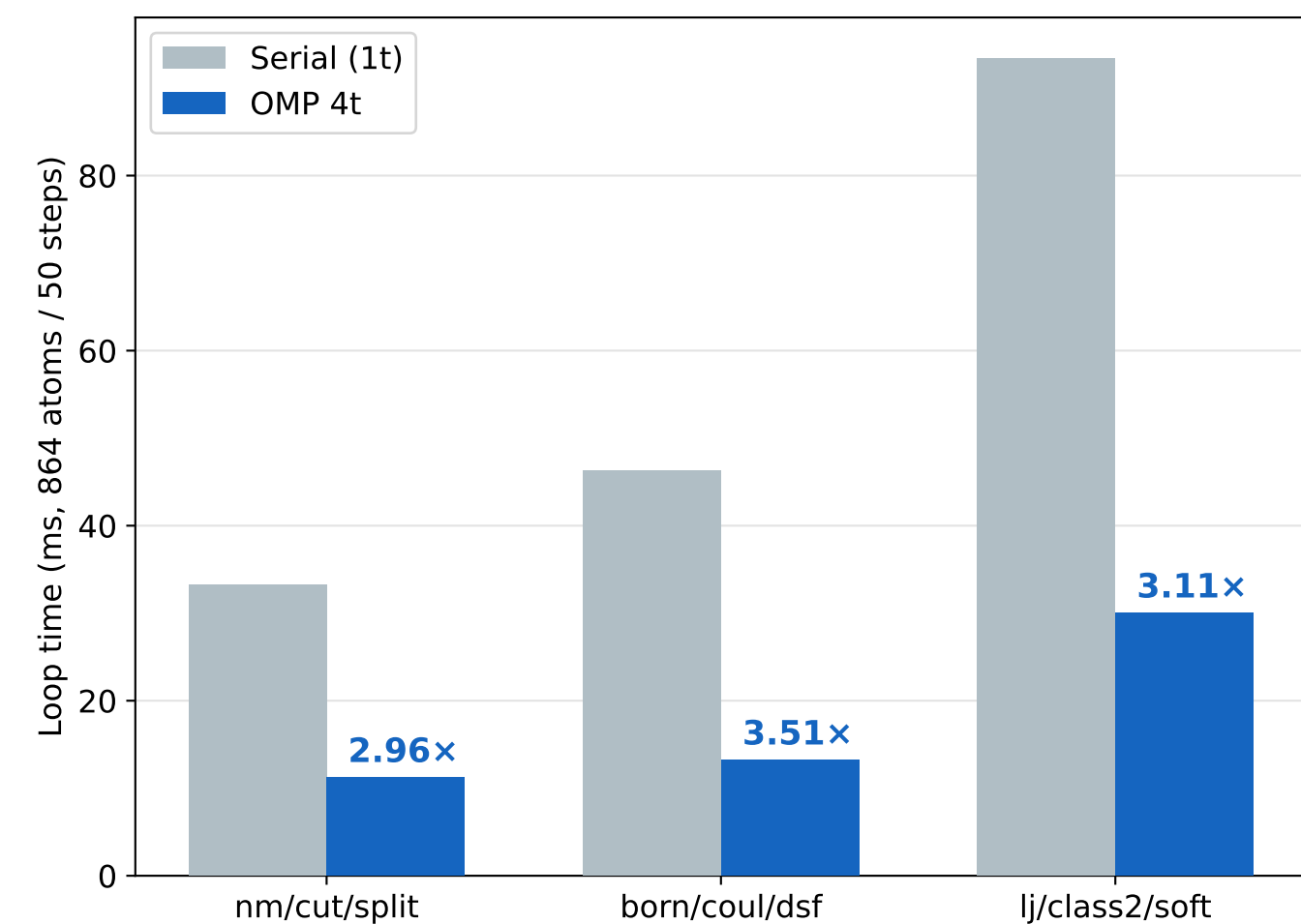
(d) Speedup for 3 newly parallelized styles (4 OMP threads vs. serial)
