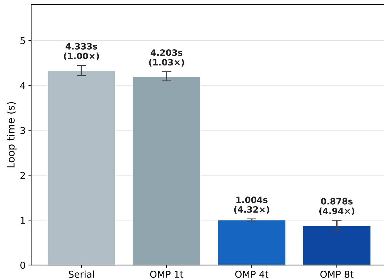
(a) Loop time vs. thread count (32,000 atoms, 500 steps, lj/cut)
