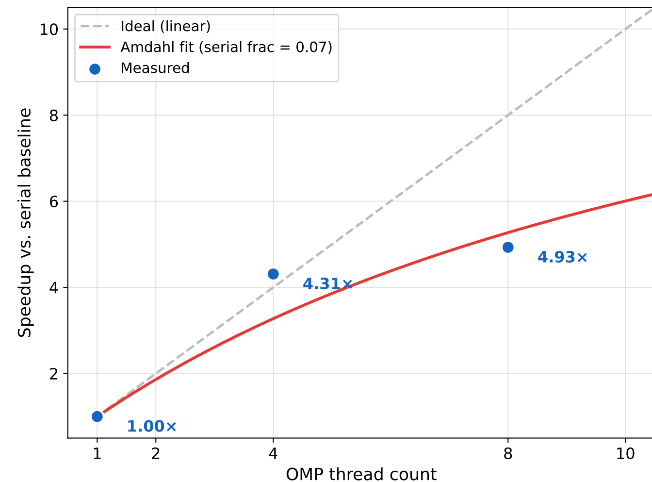
(b) Speedup scaling and Amdahl's law fit
