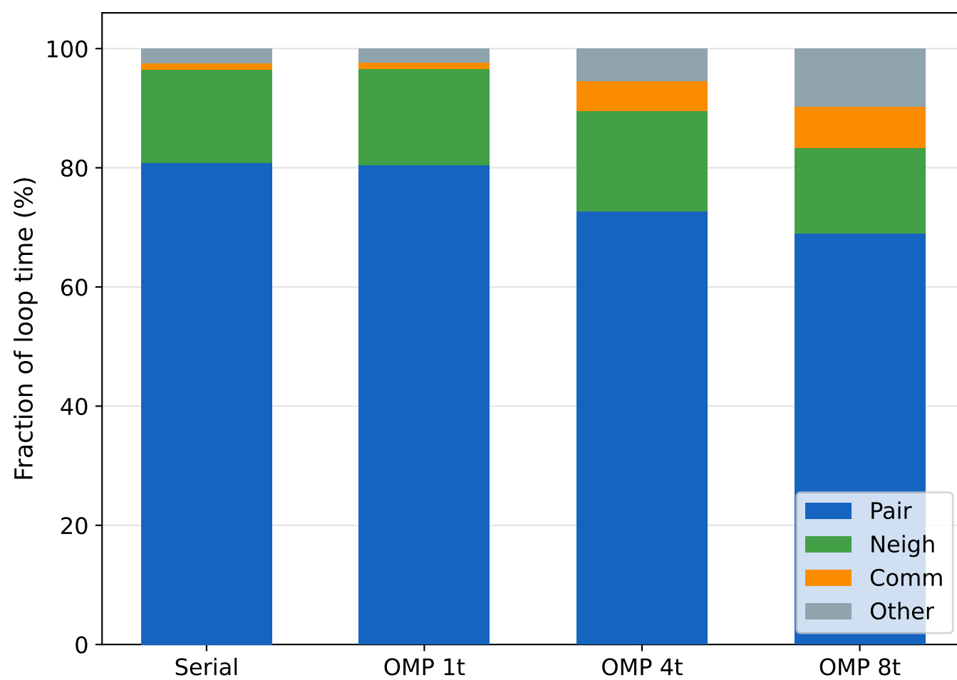
(c) Section fractions vs. thread count (Amdahl limit from non-pair sections)
