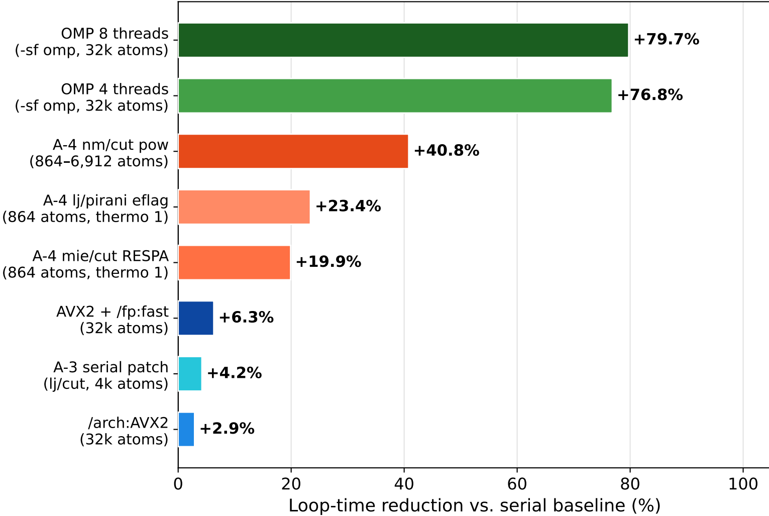
(b) Individual optimization contributions (% loop-time reduction)
