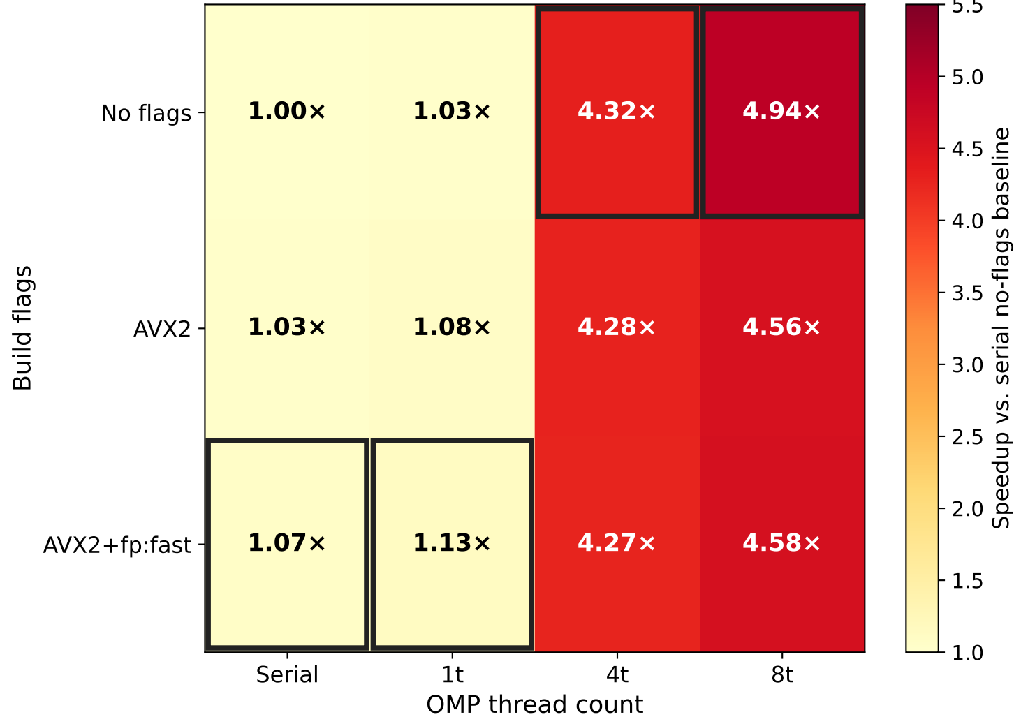
(c) Speedup heatmap — flags × threads (■ = Pareto-optimal config)
