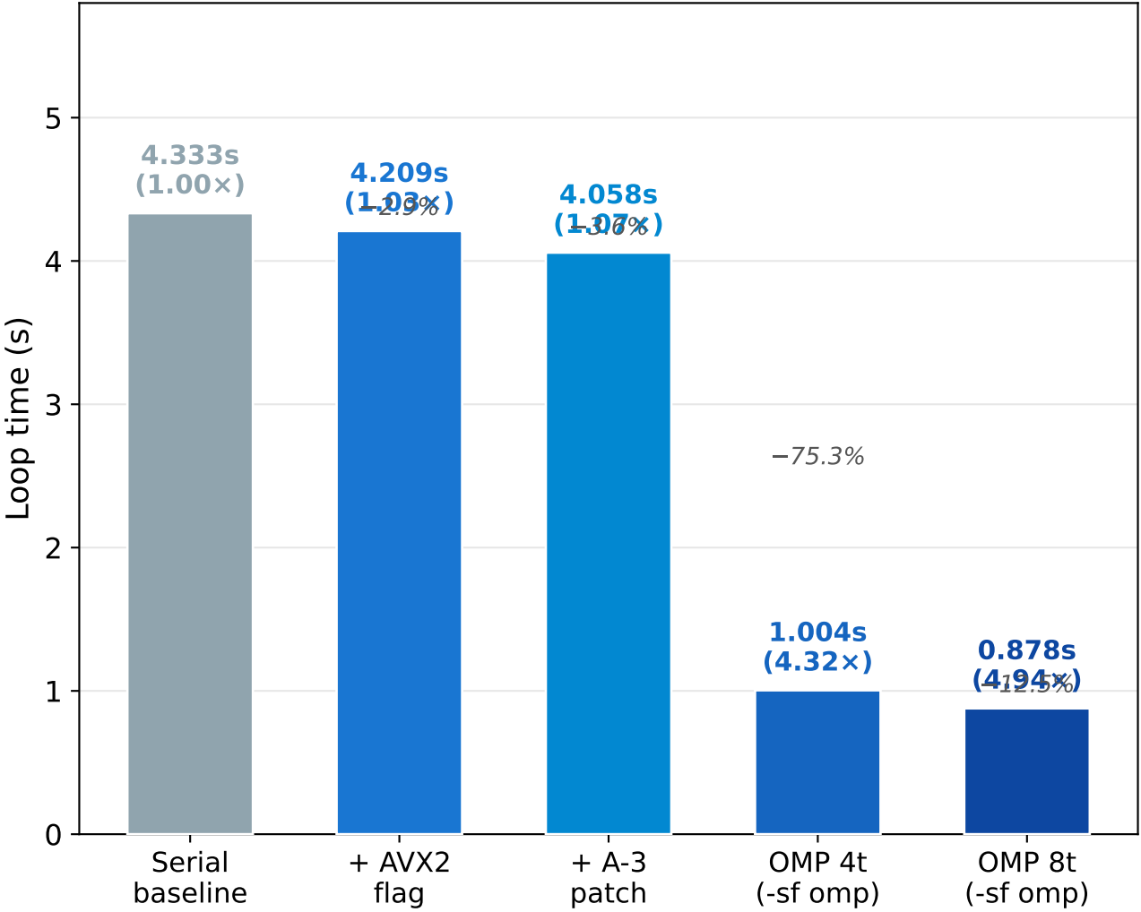
(a) Cumulative optimization waterfall (32,000 atoms, 500 steps)
